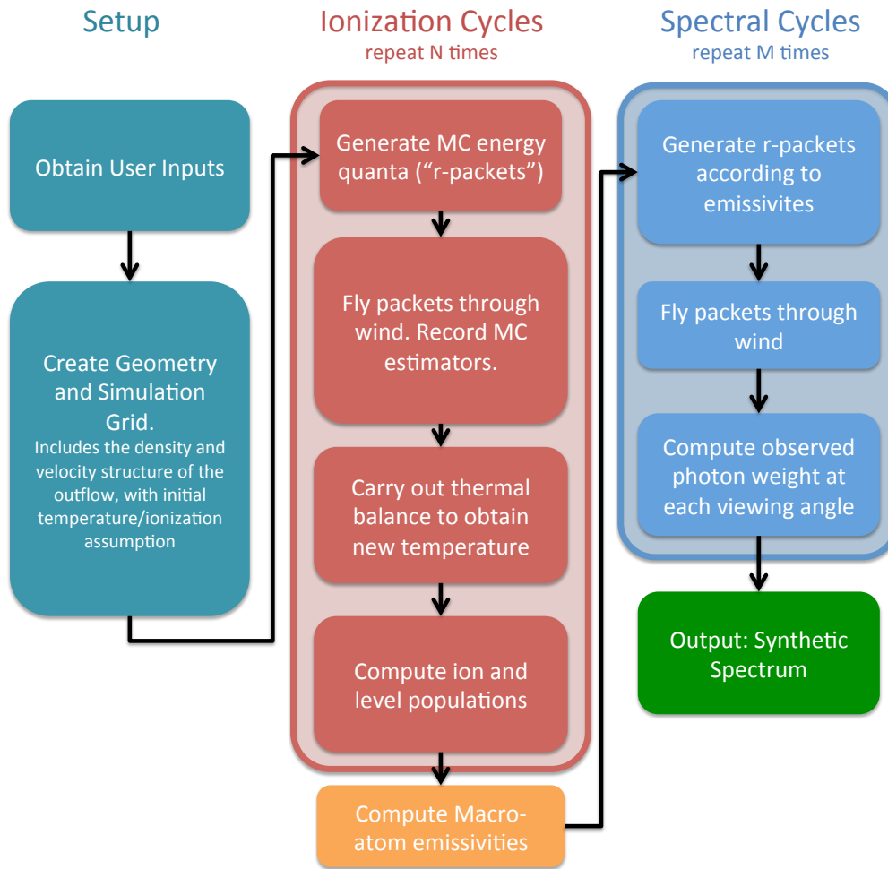
FIGURE 3.2: A flowchart showing the basic operation of PYTHON.
