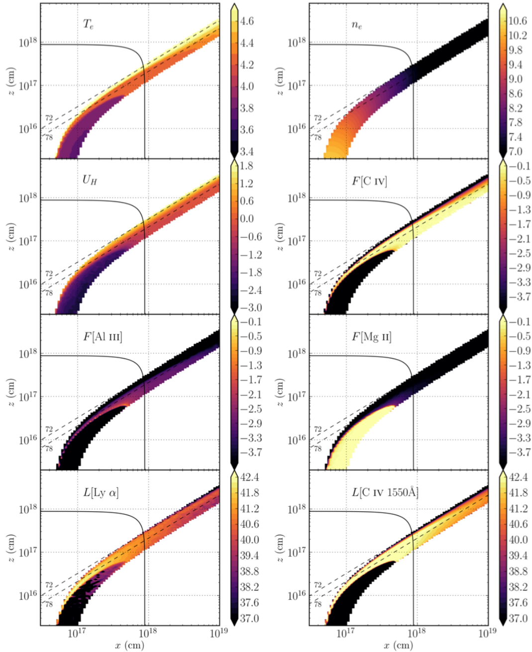
FIGURE 5.4: Contour plots showing the logarithm of some important physical properties of the outflow. The spatial scales are logarithmic and the x and z scales are not the same. The panels show the electron temperature, T_e , electron density, n_e , the ionization parameter, U_H , ion fractions, F , for three different ions and line luminosities, L , for two different lines. The line luminosities represent the luminosity of photons escaping the Sobolev region for each line. These photons do not necessarily escape to infinity. The solid black line marks a sphere at 1000 r_G . The dotted lines show the 72^\circ and 78^\circ sightlines to the centre of the system, and illustrate that different sightlines intersect material of different ionization states.
