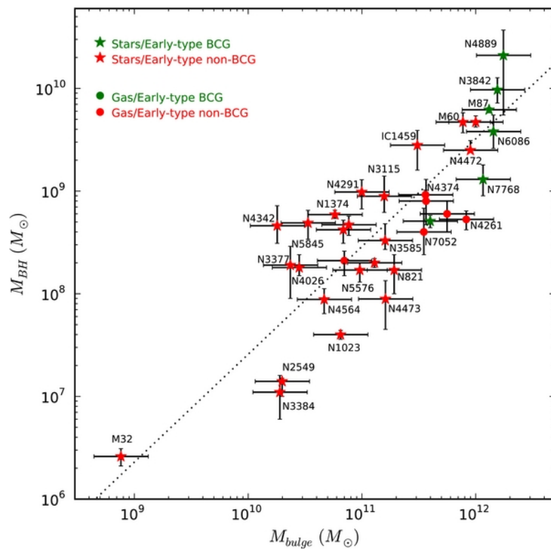
FIGURE 2.17: Credit: McConell & Ma 2013. The M_{BH} - M_{bulge} correlation.
