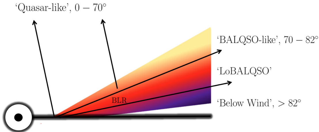
FIGURE 5.7: A cartoon describing the broad classes of sightline in the fiducial model, illustrating how geometric effects lead to the different emergent spectra. The colour gradient is approximate, but indicates the stratified ionization structure, from highly ionized (yellow) to low ionization (purple) material.
