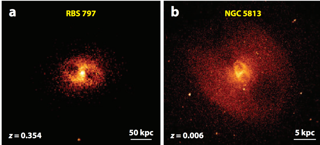
FIGURE 2.18: Figure adapted from Fabian 2012. Chandra X-ray images showing two examples of X-ray cavities, illustrating how a radio jet from an AGN can have a dramatic impact on its environment. a) The RBS 797 Cluster (Cavagnolo et al. 2011). b) elliptical galaxy NGC 5813 (Randall et al. 2011).
