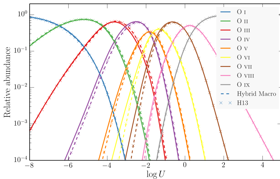
FIGURE 3.13: As figure 3.9, but for Oxygen.
