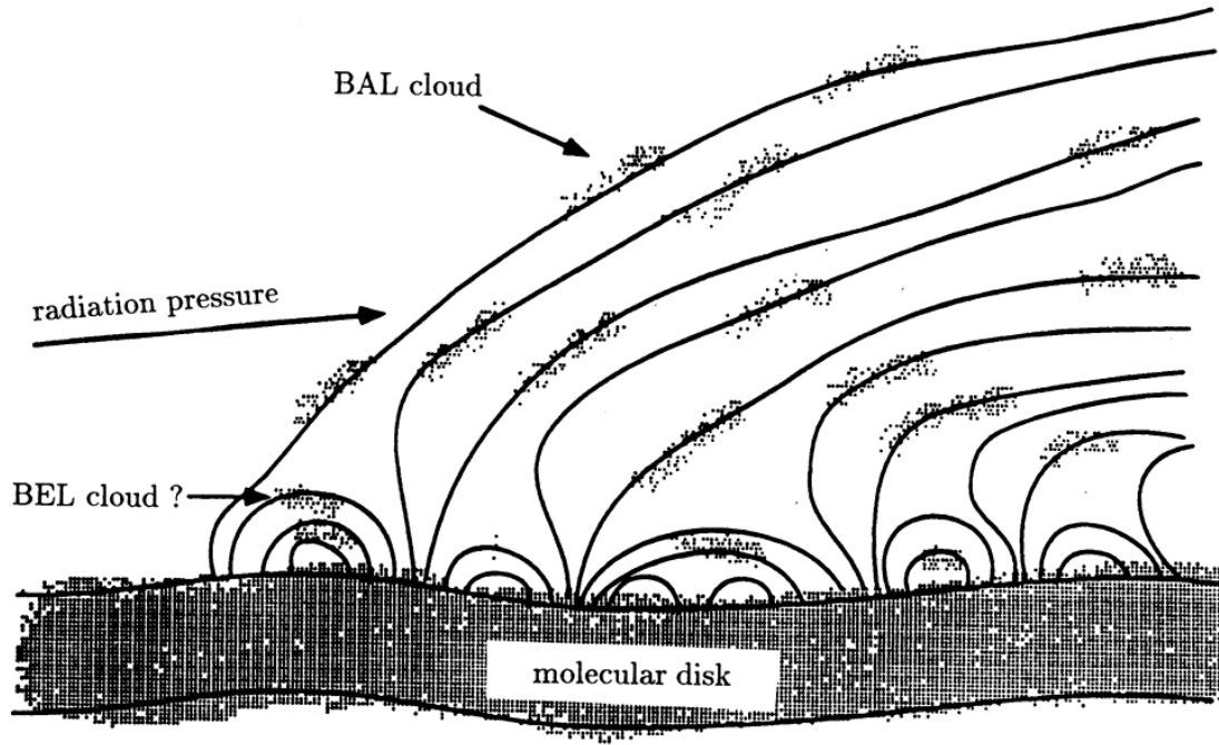
FIGURE 2.11: Credit: De Kool & Begelman 1995. A cartoon showing the components in the De Kool & Begelman model.
