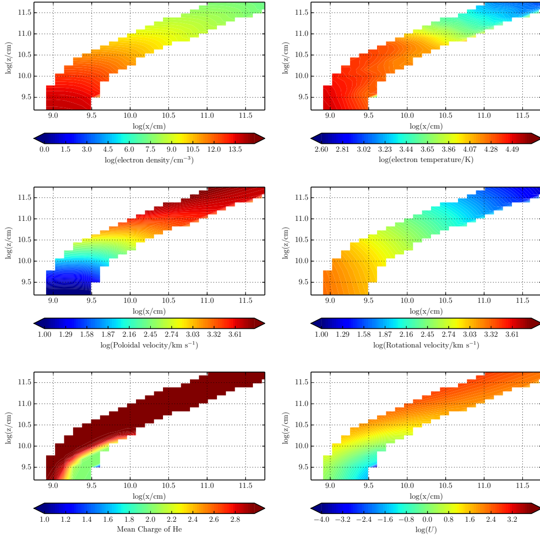
FIGURE 4.3: The physical properties of the wind – note the logarithmic scale. Near the disc plane the wind is dense, with low poloidal velocities. As the wind accelerates it becomes less dense and more highly ionized. The dominant He ion is almost always He III, apart from in a small portion of the wind at the base, which is partially shielded from the inner disc.
