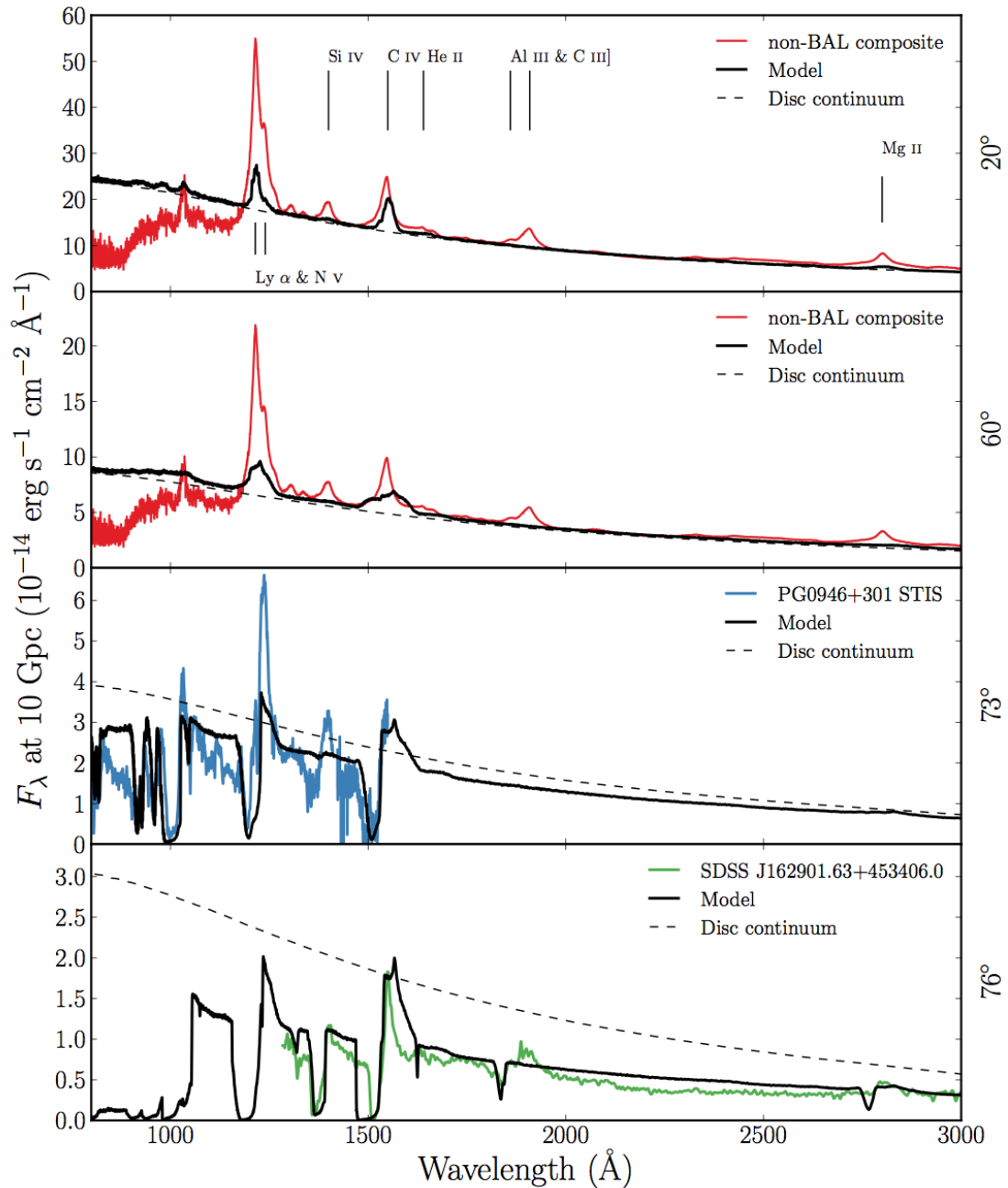
FIGURE 5.6: Synthetic spectra at four viewing angles for the fiducial model. At 20^\circ and 60^\circ I show a comparison to an SDSS quasar composite from Reichard et al. (2003). At 73^\circ and 76^\circ I show a comparison to an HST STIS spectrum of the high BALnicity BALQSO PG0946+301 (Arav et al. 2000), and an SDSS spectrum of the LoBAL quasar SDSS J162901.63+453406.0, respectively. The dotted line shows a disc only continuum to show the effect of the outflow on the continuum level. All the spectra are scaled to the model flux at 2000 \text{ \AA} , except for the HST STIS spectrum of PG0946+301, which is scaled to 1350 \text{ \AA} due to the incomplete wavelength coverage.
