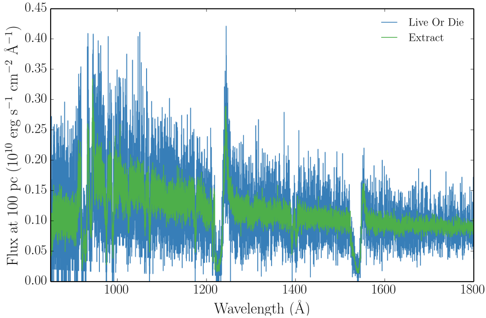
FIGURE 3.7: A synthetic spectrum after 30 spectral cycles with 100,000 photons from simple CV wind model at a 60^\circ viewing angle. Spectra produced with both the extract and live or die modes are shown. The effectiveness of the extract variance reduction technique can be clearly seen, and we can see that the spectral shape is unaltered.
