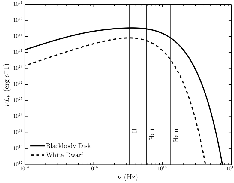
FIGURE 4.2: The spectral energy distribution of the accretion disc and white dwarf used in the ionization cycles for the CV modelling. The important ionization edges for hydrogen and helium are marked.
