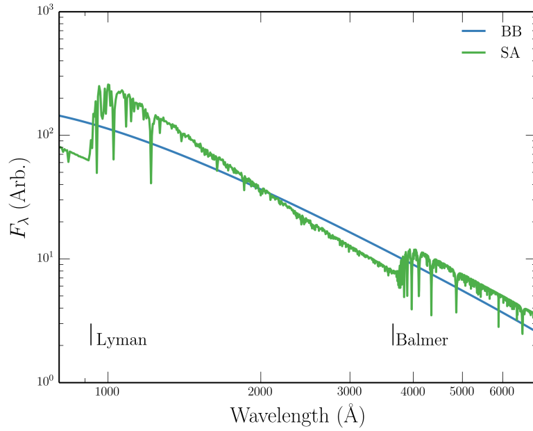
FIGURE 1.5: A comparison between a disc spectrum computed with stellar atmosphere models and standard multi-temperature blackbody disc. The major photoabsorption edges are marked. Flux is reprocessed into different wavelengths by bound-free opacities, and line blanketing also has a big effect on the spectrum. The Hydrogen and Helium lines also experience a degree of pressure broadening.
