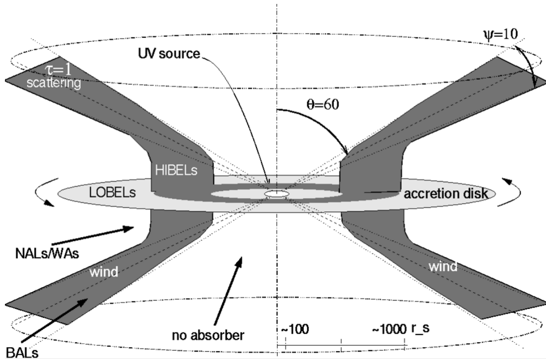
FIGURE 2.12: Credit: Martin Elvis. A schematic showing the main features of the Elvis model. A biconical wind rises from an accretion disc, and the observed spectrum is determined purely by the viewing angle of the observer.
