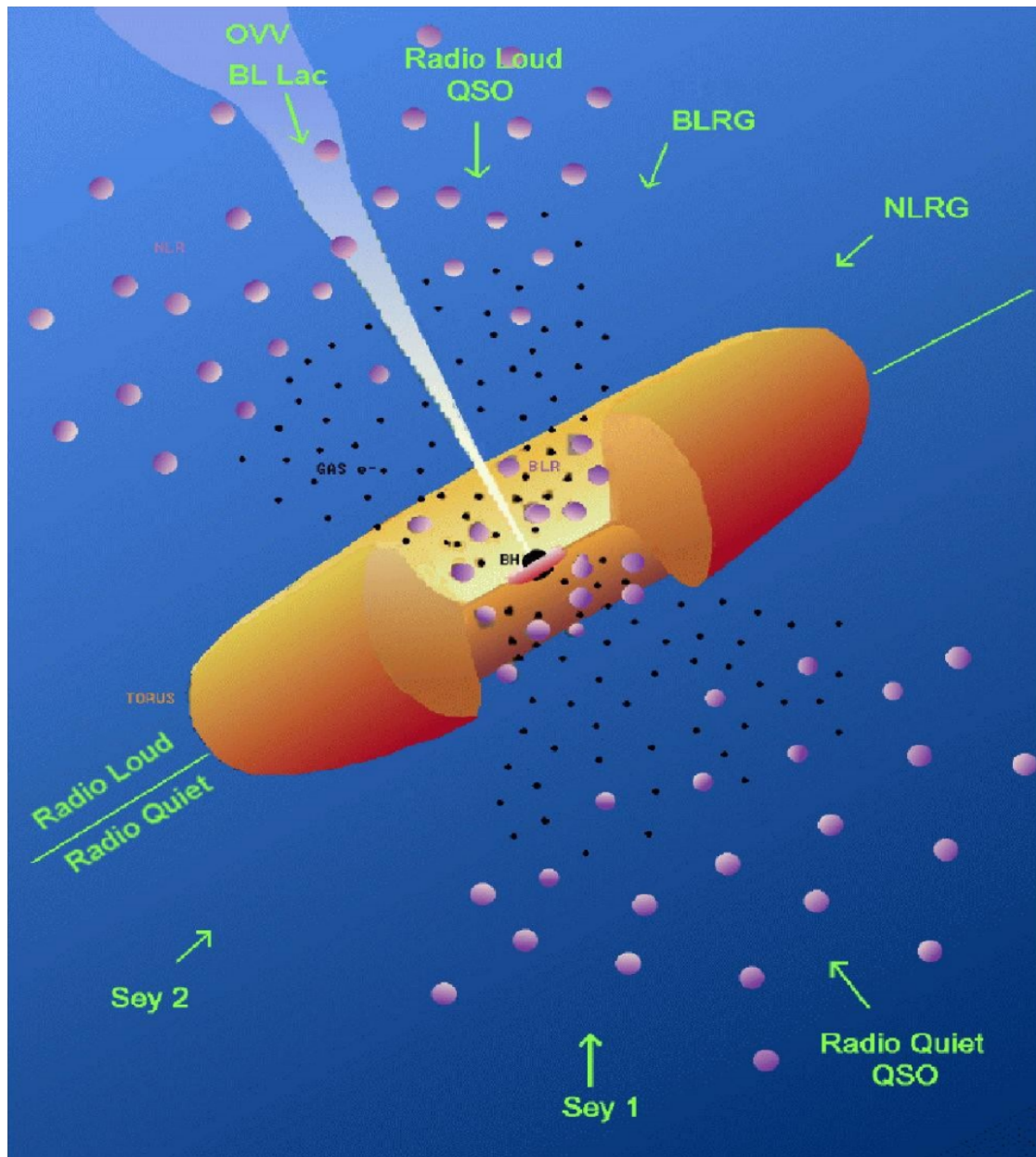
FIGURE 1.13: A unified scheme for AGN. The broad line region is compact and can thus be obscured from view by a dusty torus, whereas the larger narrow line region is always visible. The radio-loud/radio-quiet dichotomy is explained by the presence or absence of a radio jet.
