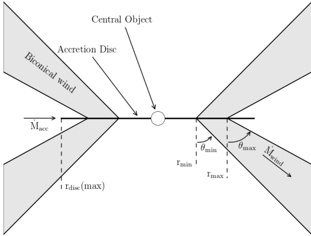
FIGURE 2.14: A schematic showing the geometry and kinematics of the SV93 model.
