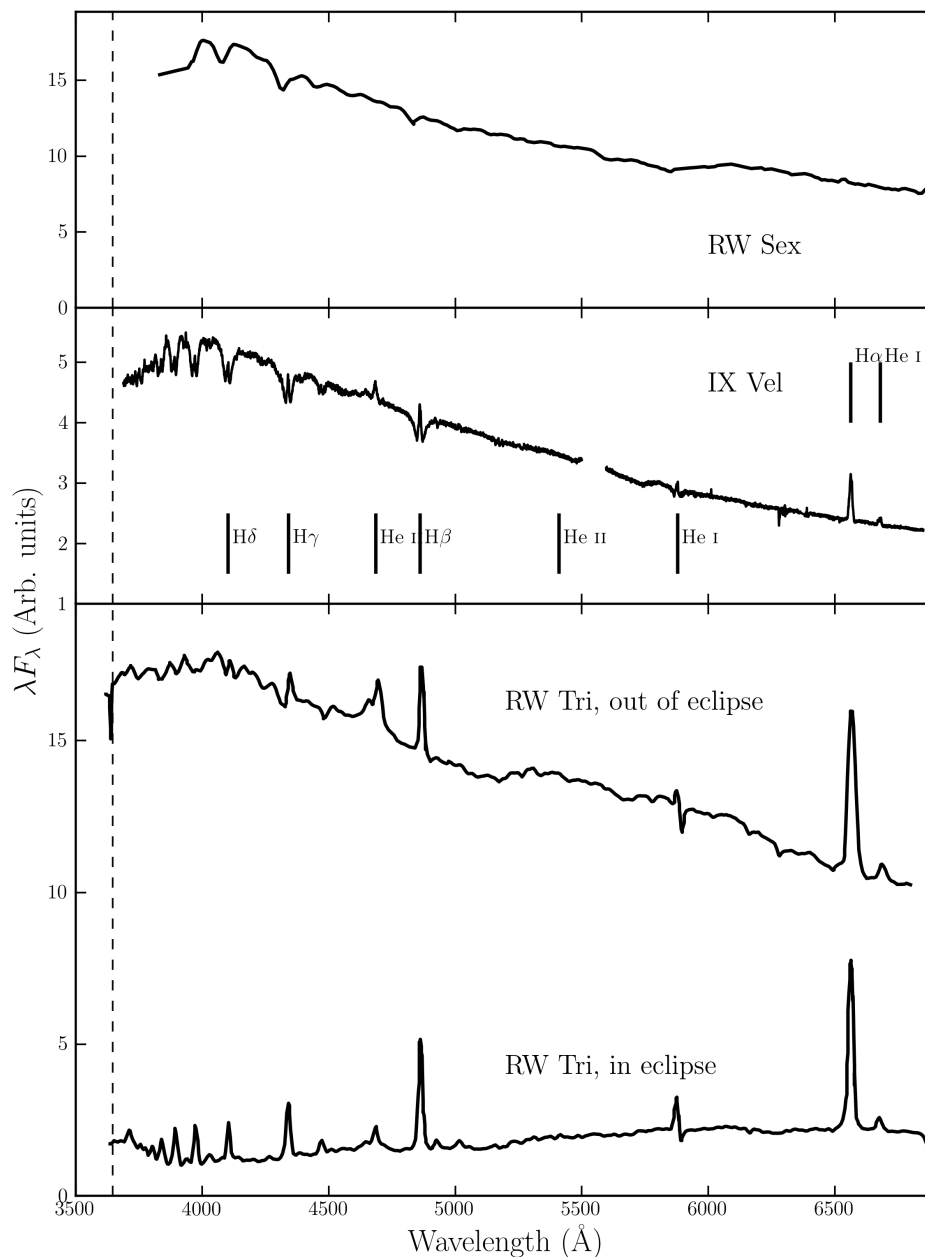
FIGURE 1.11: Optical spectra of three nova-like variables: RW Sex (top; Beuermann et al. 1992), IX Vel (top middle; A. F. Pala & B. T. Gaensicke, private communication) and RW Tri in and out of eclipse (bottom two panels; Groot et al. 2004). The data for RW Sex and RW Tri were digitized from the respective publications, and the IX Vel spectrum was obtained using the XSHOOTER spectrograph on the Very Large Telescope on 2014 October 10. These systems have approximate inclinations of 30^\circ , 60^\circ and 80^\circ respectively. The trend of increasing Balmer line emission with inclination can be seen. In RW Tri strong single-peaked emission in the Balmer lines is seen even in eclipse, indicating that the lines may be formed in a spatially extensive disc wind, and there is even a suggestion of a (potentially wind-formed) recombination continuum in the eclipsed spectrum. I have attempted to show each spectrum over a similar dynamic range.
