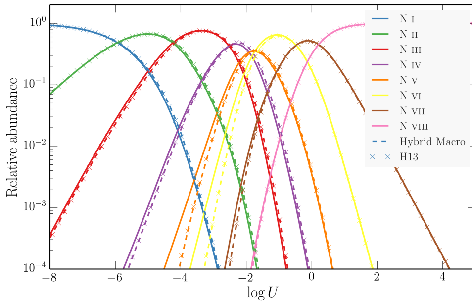
FIGURE 3.12: As figure 3.9, but for Nitrogen.
