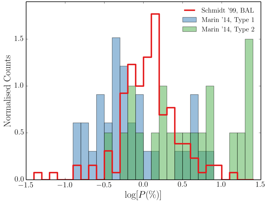
FIGURE 6.12: Histograms of polarisation percentages for BAL quasars from Schmidt et al. (1999) together with the Marin et al. (2014) AGN sample.
