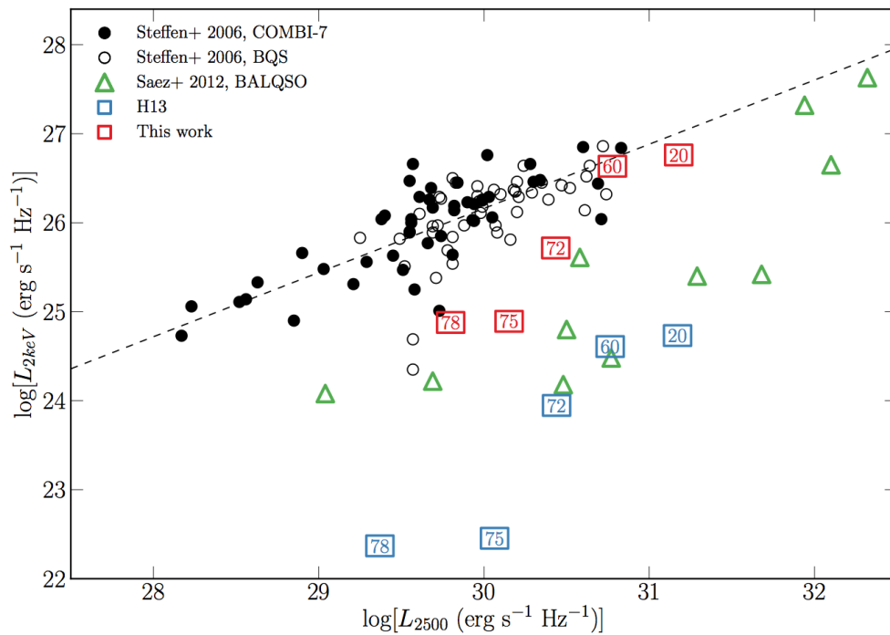
FIGURE 5.9: X-ray (2 keV) luminosity of the clumped model (red squares) and the H13 model (blue squares), plotted against monochromatic luminosity at 2500 Å. The points are labeled according to inclination; angles > 70^\circ correspond to BALs in this scheme (see Fig. 5.7). Also plotted are measurements from the COMBI-7 AGN and the BQS samples (Steffen et al. 2006) and the Saez et al. (2012) sample of BALQSOs. The dotted line shows the best fit relation for non-BALQSOs from Steffen et al. (2006).
