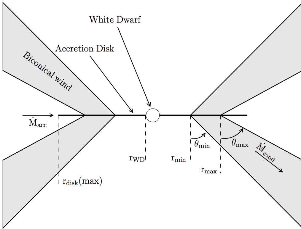
FIGURE 4.1: Cartoon illustrating the geometry and kinematics of the benchmark CV wind model.
