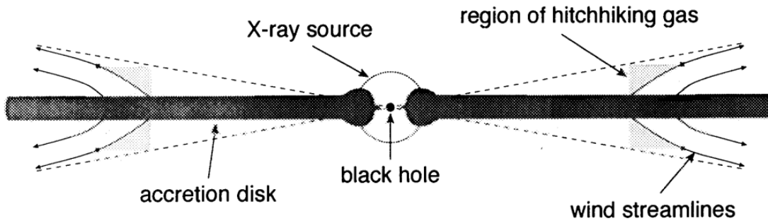
FIGURE 2.10: Credit: Murray et al. 1995. Cartoon showing the geometry of the MCGV95 model.
