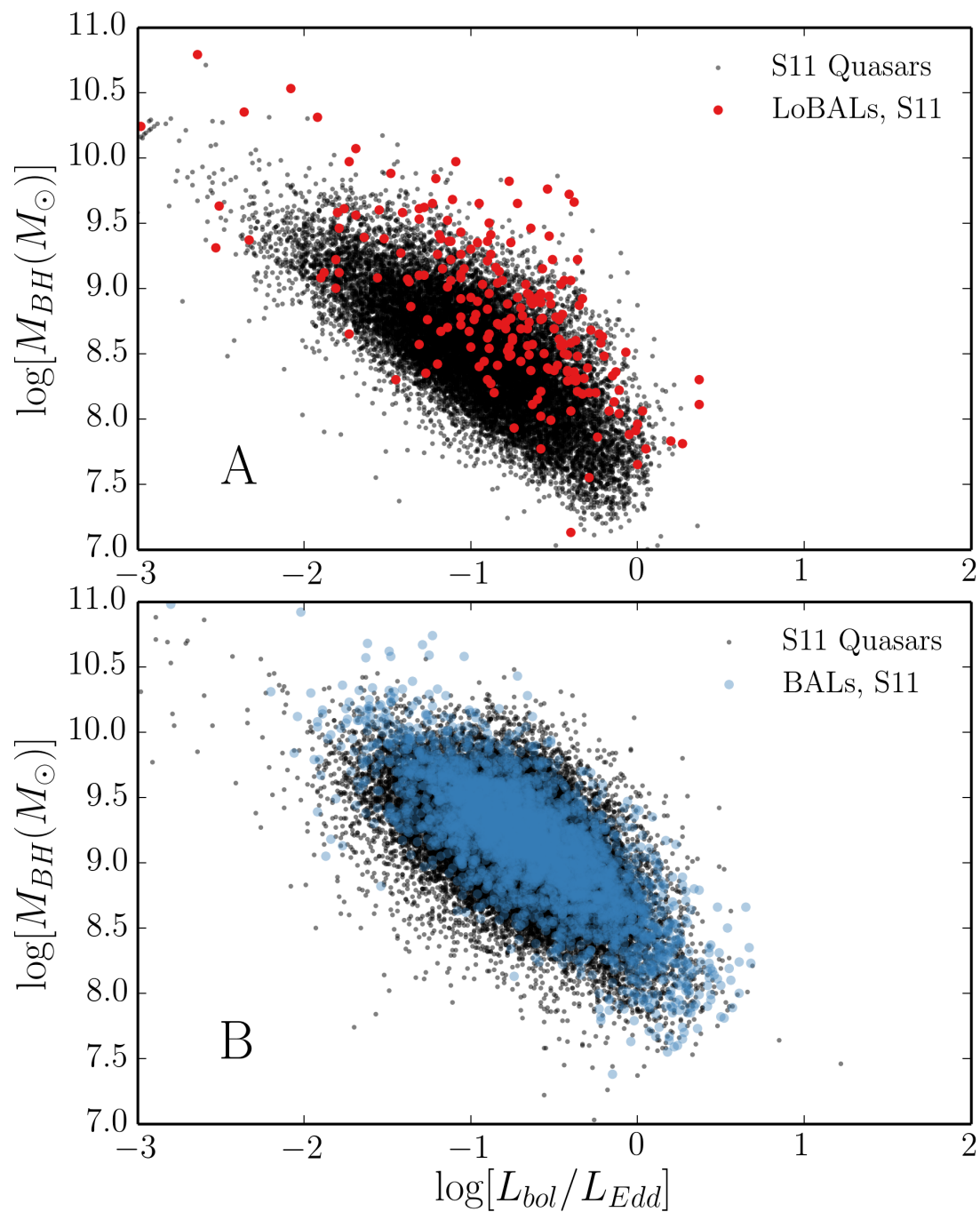
FIGURE 6.1: BH mass and Eddington fraction measurements from S11 for Sample A (top) and Sample B (bottom). The LoBALQSOs in sample A and BALQSOs in Sample B are also plotted in each case.
