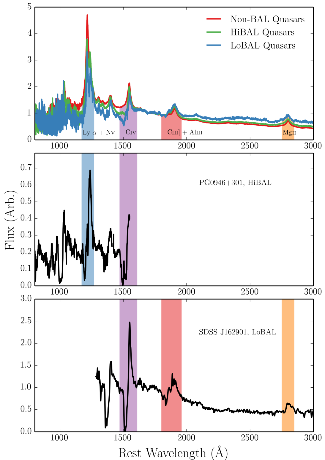
FIGURE 2.7: Top Panel: A comparison between the SDSS non-BAL, HiBAL and LoBAL composite spectra as presented in Reichard et al. (2003). Bottom Two Panels: Two individual examples of a HiBAL and LoBAL quasar spectrum, respectively. In all panels some of the more prominent lines are labeled and shaded, and the object name is given in the bottom two plots.
