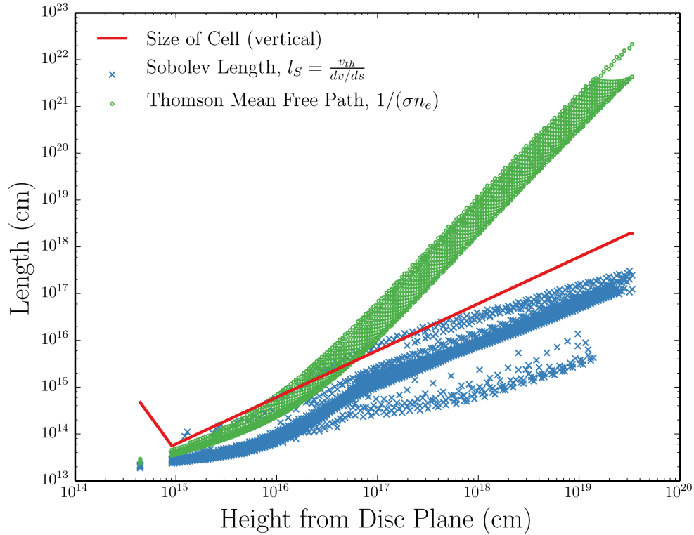
FIGURE 5.3: Some typical length scales for the fiducial model. This places a formal limit of \sim 10^{12} cm on clump sizes in the microclumping framework, and confirms that the cells are sufficiently larger than the Sobolev length in almost all cases.
