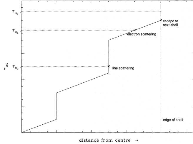
FIGURE 3.3: Credit: Mazzali & Lucy 1993. The process of choosing a scattering location in a cell.
