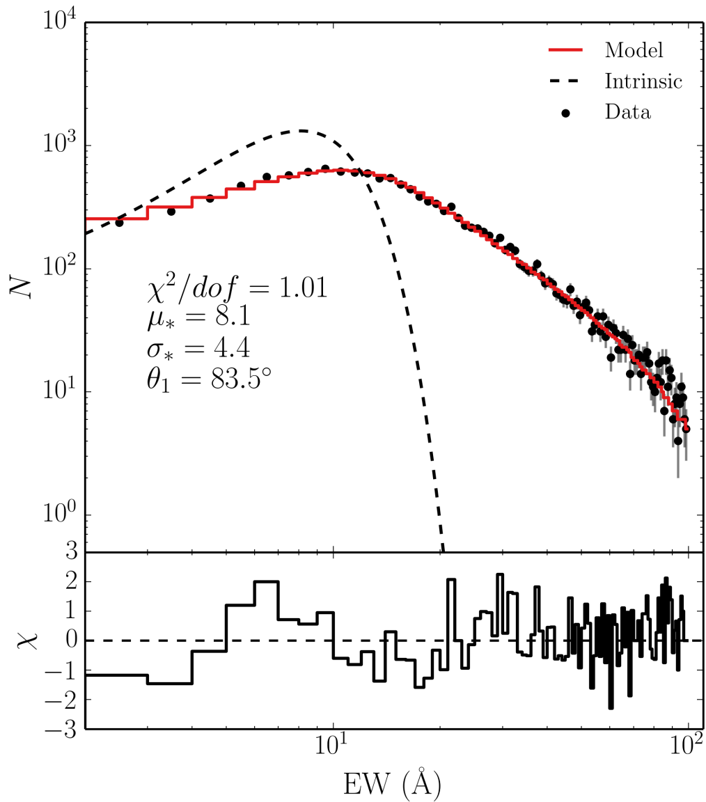
FIGURE 6.5: The EW[O III] distribution of quasars in the R11 sample (black points), with \sqrt{N} errorbars, and the best fit model with a maximum viewing angle of 84^\circ . The intrinsic Gaussian distribution is shown with a dashed line. The plotted data is equivalent to the non-BAL histogram in the top left panel of Fig. 6.2, except that it uses linear binning and adopts the R11 sample criteria rather than using sample A.
