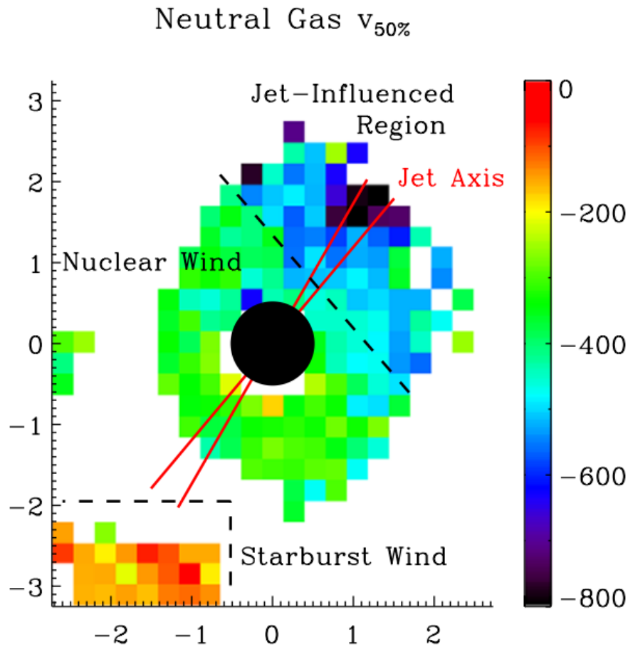
FIGURE 2.19: Credit: Rupke & Veilleux 2011. Results of Gaussian line profile fitting to integral field spectroscopy of Mrk 231. The quantity shown, v_{50\%} , corresponds to the centre of the fitted Gaussian profile and indicates that high outflow velocities are present in the neutral gas.
