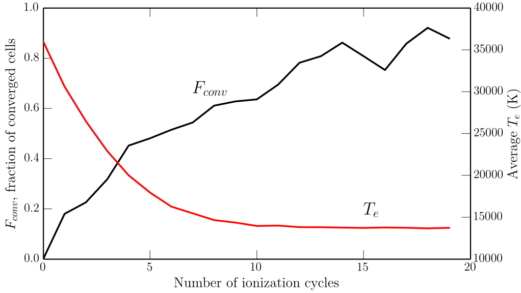
FIGURE 3.6: The average temperature and fraction of converged cells in a typical CV model, shown as a function of the number of ionization cycles completed.
