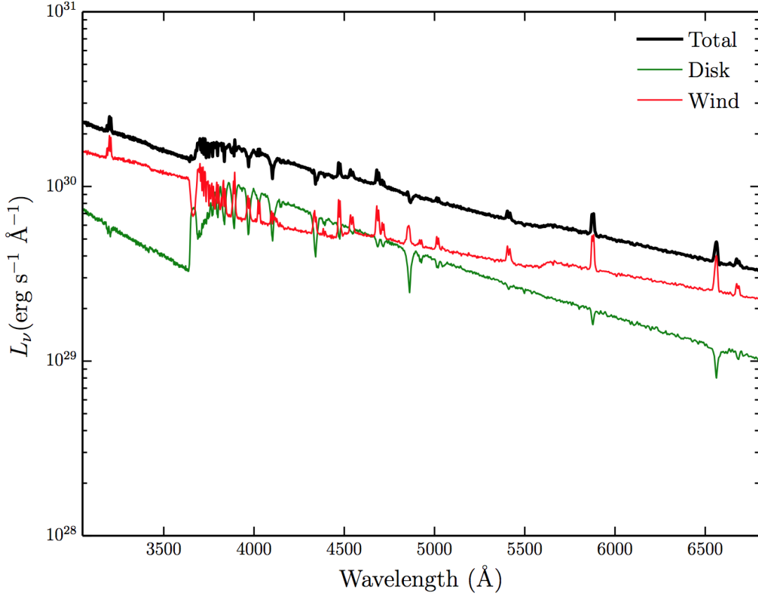
FIGURE 4.9: Total packet-binned spectra across all viewing angles, in units of monochromatic luminosity. The thick black line shows the total integrated escaping spectrum, while the green line shows disc photons which escape without being reprocessed by the wind. The red line show the contributions from reprocessed photons. In this denser model the reprocessed contribution is significant compared to the escaping disc spectrum. The Balmer continuum emission is prominent, and the wind has a clear effect on the overall spectral shape.
