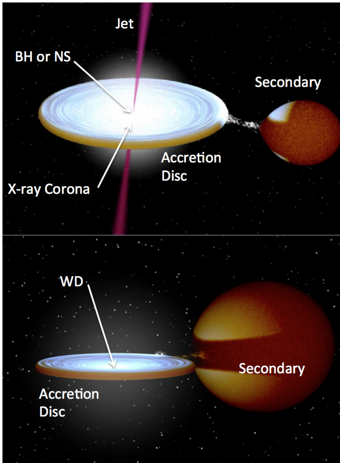
FIGURE 1.6: Credit: Rob Hynes. Artist's impression of a low-mass X-ray binary (top) and cataclysmic variable (bottom). The key components are marked, and the clear similarity in overall structure is apparent.
