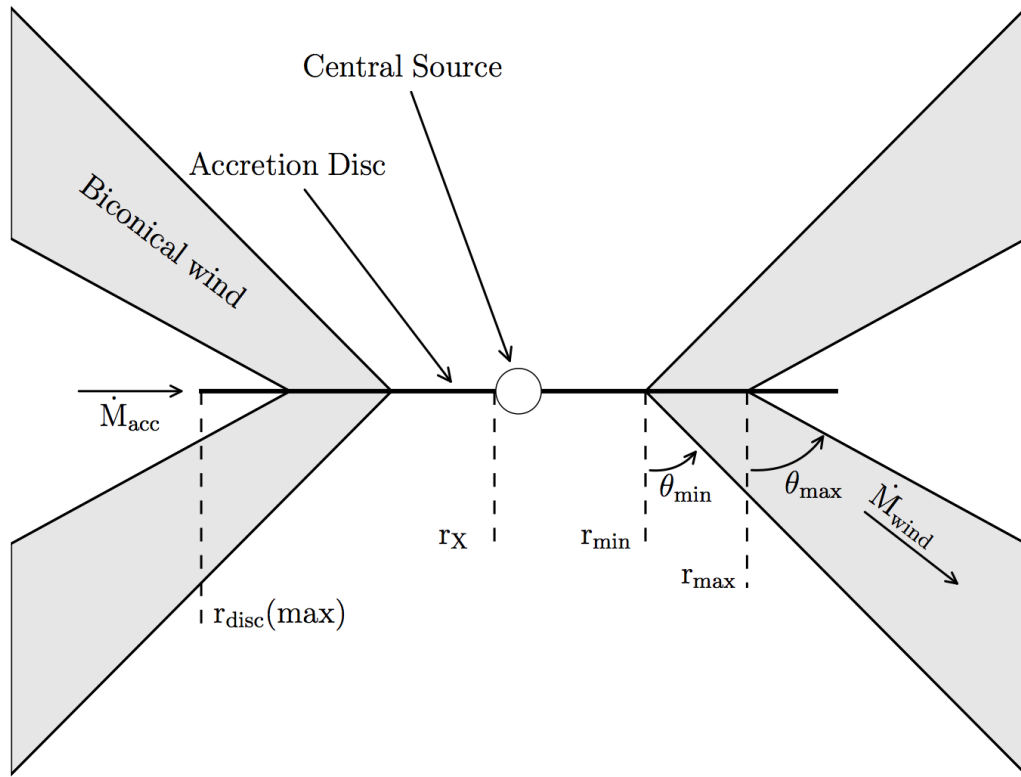
FIGURE 5.1: A cartoon showing the geometry and some key parameters of the biconical quasar wind model.
