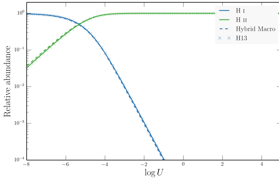
FIGURE 3.9: Relative ion fractions as a function of ionization parameter from the hybrid macro-atom scheme, with Hydrogen and Helium treated as a full macro-atom (dotted lines), compared to both CLOUDY (solid lines) and PYTHON in simple-atom only mode (H13, crosses). The colours correspond to the different ionic stages and are labeled for the CLOUDY case.
