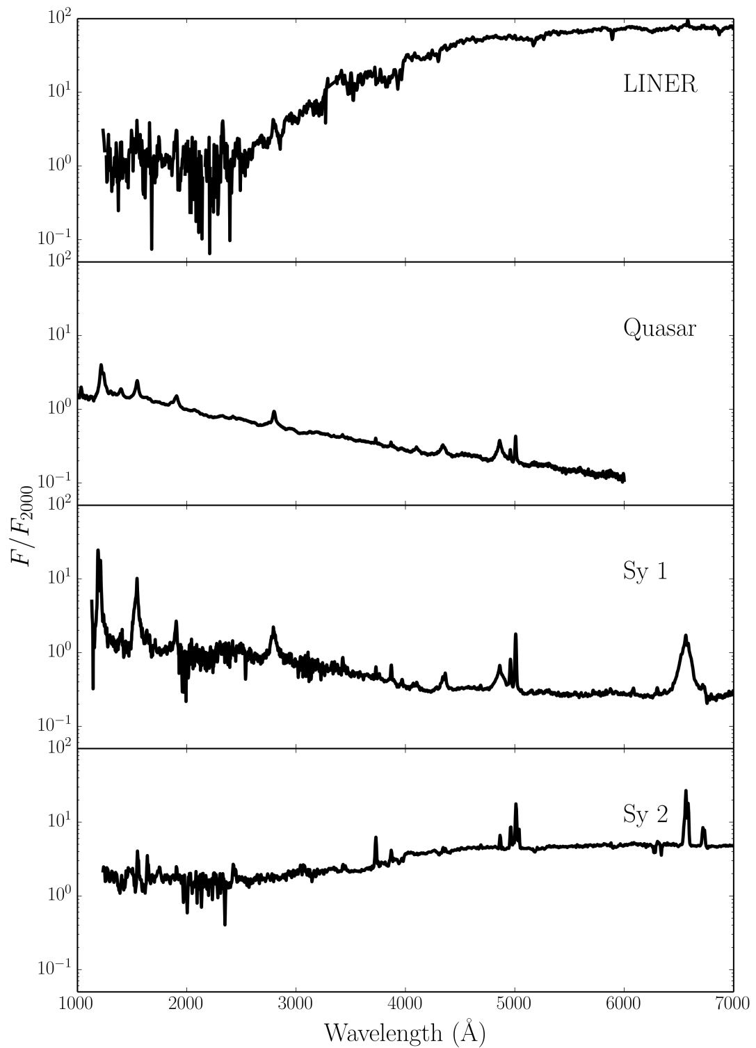
FIGURE 1.12: Template spectra, from the AGN atlas, for four common types of AGN. Obtained from http://www.stsci.edu/hst/observatory/crds/cdbs_agn.html .
