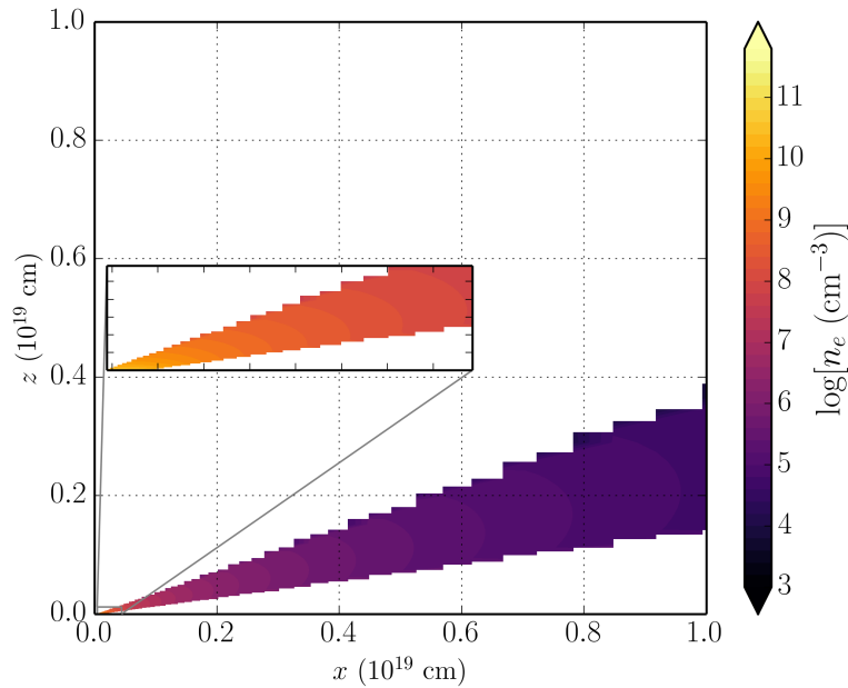
FIGURE 5.5: The electron density in the model, this time on linear axes in order to illustrate the density contrasts and scale of the system. The plot is on the scale of the acceleration length, whereas the inset is a box of 2700 \times 800 r_G , where the bottom left corner corresponds to the base of the innermost streamline.
