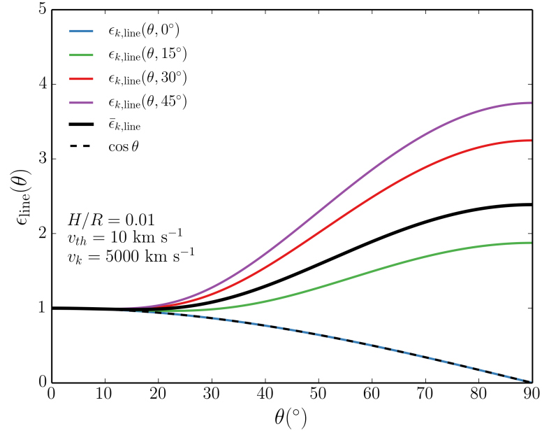
FIGURE 6.14: The line angular emissivity function from a Keplerian disc as a function of inclination angle, \theta , for a few different azimuthal angles, \phi . The azimuthally-averaged case, \bar{\epsilon}_{k,\text{line}} (thick black line), and the zero Keplerian velocity shear case, \epsilon_{0,\text{line}}(\theta) = \cos \theta (dotted line), are also shown.
