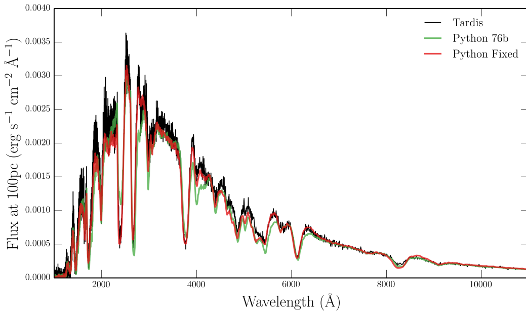
FIGURE 3.16: Comparison between TARDIS and PYTHON synthetic spectra from a simple 1D supernova model. A bug in Doppler shifting of photons was discovered around PYTHON 76, meaning that the code now gives even better agreement than presented in Kerzendorf & Sim 2014.
