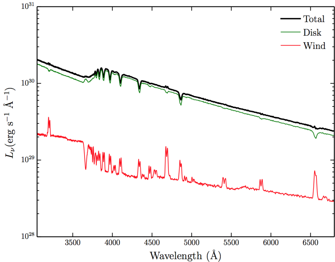
FIGURE 4.6: Total packet-binned spectra across all viewing angles, in units of monochromatic luminosity. The thick black line shows the total integrated escaping spectrum, while the green line shows disc photons which escape without being reprocessed by the wind. The red line shows the contributions from reprocessed photons. Recombination continuum emission blueward of the Balmer edge is already prominent relative to other wind continuum processes, but is not sufficient to fill in the Balmer jump in this specific model.
