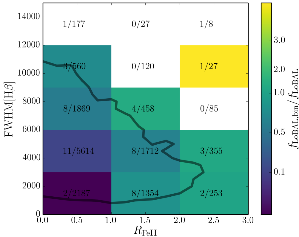
FIGURE 6.11: LoBAL fraction compared to global LoBAL fraction in Eigenvector 1 space, in bins of \Delta R_{\text{FeII}} = 1 and \Delta \text{FWHM}[\text{H}\beta] = 3000 \text{ km s}^{-1} . The contour shows the outermost contour from Fig. 6.10 for reference. The text shows N_{\text{LoBAL}}/N_{\text{non-BAL}} , where N_{\text{LoBAL}} is the number of LoBALQSOs in the bin and N_{\text{non-BAL}} in the number of non-BAL quasars in the bin.
