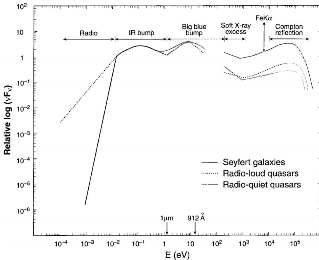
FIGURE 1.14: Credit: Koratkar & Blaes 1999 Approximate average broadband SEDs for a few types of AGN. The series of characteristic bumps can be clearly seen. The Soft-X-ray excess is also visible (see section 1.3.2.1).
