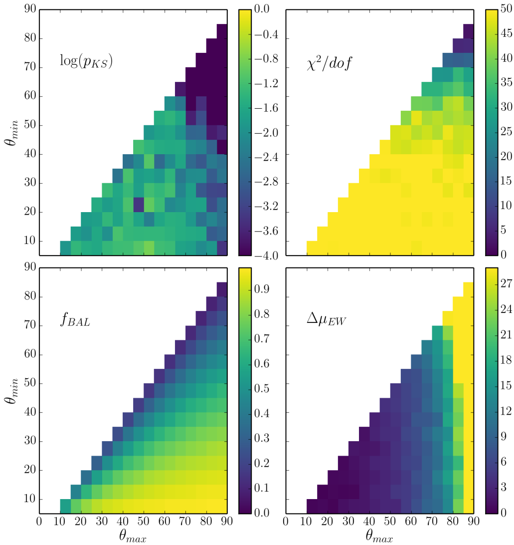
FIGURE 6.8: Heat map showing the results of the MC simulation described in section 6.4.2. The quantities shown are discussed further in the text, but correspond to (clockwise from top left): the p_{KS} value from a comparison between the mock BAL dataset and the observed BAL dataset, the reduced \chi^2 from the fit to the non-BAL EW distribution, the difference in mean EW between the mock BAL and mock non-BAL datasets, and the BAL fraction expected for the geometry in question.
