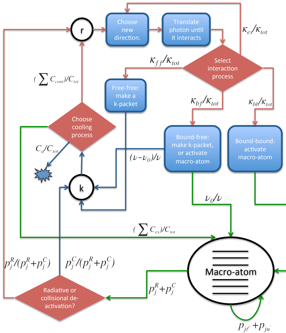
FIGURE 3.4: The decision tree traversed by an energy packet in macro-atom mode, depicting the interaction between radiation ( r -packets), the thermal pool ( k -packets), and ionization and ionization/excitation energy (macro-atoms). The probabilities at each decision point are marked, and are defined in the text. The red, blue and green coloured arrows represent radiant, kinetic and ionization/excitation energy respectively. The symbols are defined in the text, except C_{cont} and C_{ex} which refer to cooling contributions to radiative and excitation energy respectively.
