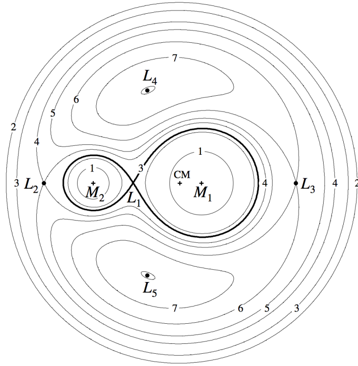
FIGURE 1.7: Credit: Frank et al. 2002. The Roche potential in a binary system for q_M = M_2/M_1 = 0.25 . The Lagrangian points are marked, as are the locations of the individual and system centres of mass.
