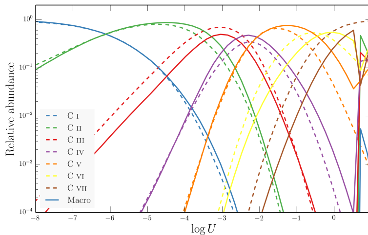
FIGURE 7.1: Ion fractions as a function of ionization parameter when Carbon is treated as a simple-atom (dotted lines) or macro-atom (solid lines) Although serious, as yet unsolved, numerical problems appear at high ionization parameters, the fundamental machinery for treating Carbon as a macro-atom is now in place.
