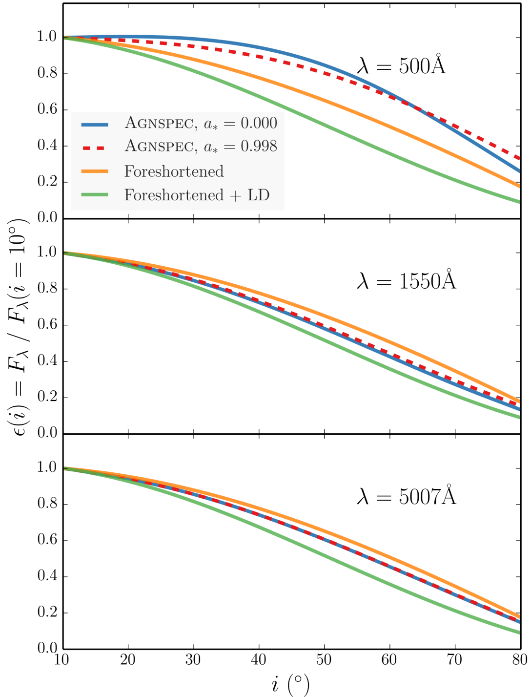
FIGURE 6.3: Angular variation of continuum luminosity from AGNSPEC and classical thin disc models. The monochromatic continuum luminosities is divided by the monochromatic continuum luminosity at 10^\circ , from AGNSPEC and classical thin disc models, at three different wavelengths. The models are computed for an Eddington fraction of 0.2 and M_{BH} = 10^9 M_\odot . In each panel I show both Kerr and Schwarzschild AGNSPEC models, and the classical models are for both pure foreshortened discs and foreshortened and limb darkened (LD) discs.
