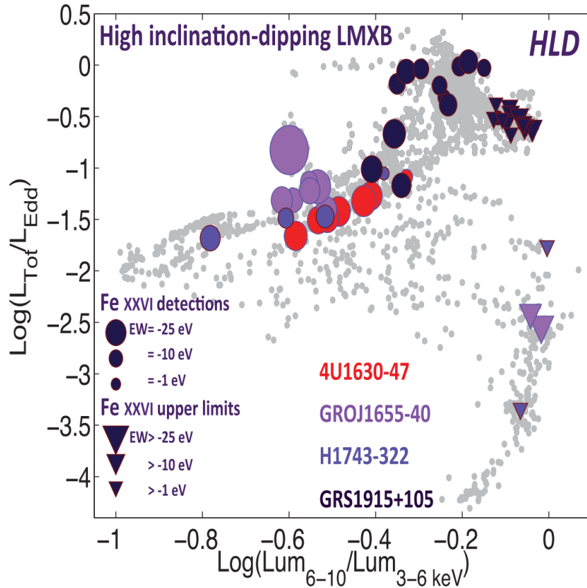
FIGURE 2.6: Credit: Ponti et al. 2012. Hardness-luminosity diagram for four dipping LMXBs, demonstrating that winds appear only in the soft state. The points are colour-coded by system, and are shown against the background grey points of all LMXBs studied by Ponti et al. (2012). None of the low inclination sources in their sample show Fe xxvi absorption detections.
