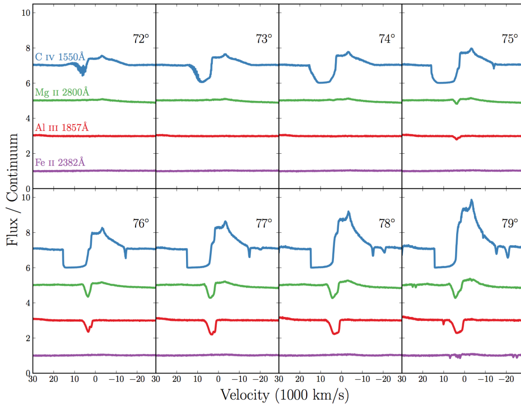
FIGURE 5.10: C IV, Mg II, Al III and Fe II line profiles for viewing angles from 72 – 79°. The profiles are plotted relative to the local continuum with an offset applied for clarity. Lower ionization profiles appear at a subset of high inclinations, compared to the ubiquitous C IV profile.
