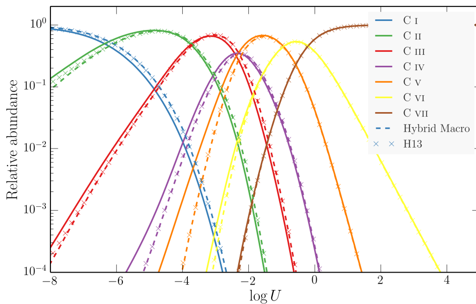
FIGURE 3.11: As figure 3.9, but for Carbon.
