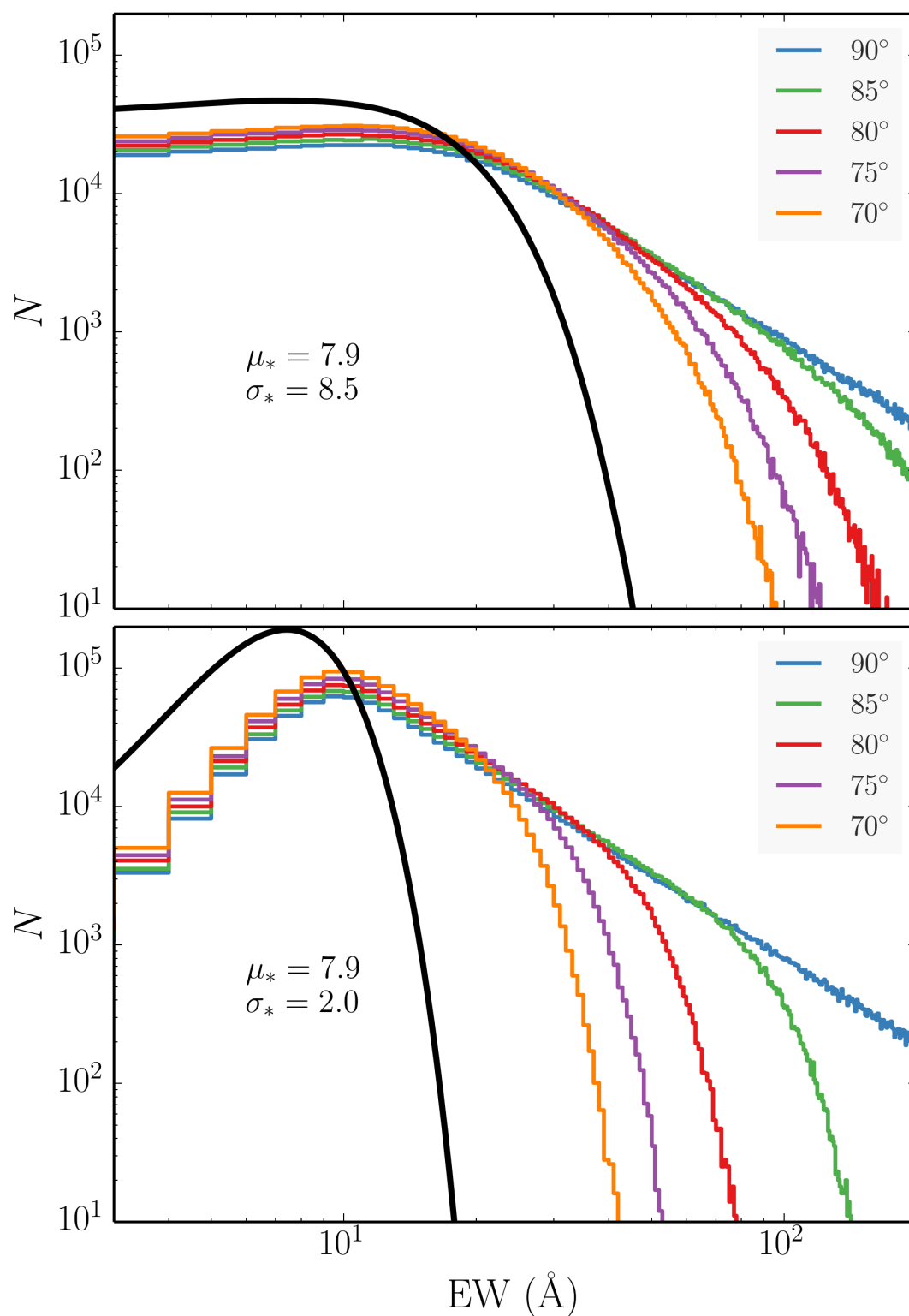
FIGURE 6.4: Theoretical EW distributions from the numerical experiment described in section 6.4.1 for a few different maximum angles. The results in the top panel use the same intrinsic distribution as Model 1 from R11 (shown in black), whereas the bottom panel shows the distributions obtained from a narrower intrinsic Gaussian. By the time the maximum angle is limited to around 70^\circ the cutoff is clear even at moderate values of EW.
