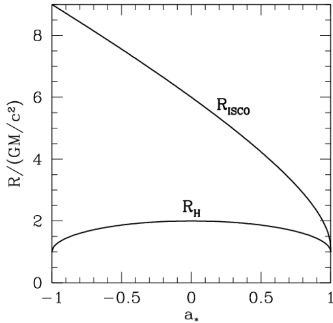
FIGURE 1.3: Credit: Narayan 2014. The radius of the ISCO, R_{ISCO} , and the horizon, R_H , is as a function of the BH spin parameter, a_* . a_* = 0 corresponds to a Schwarzschild BH, and a_* = 1 and a_* = -1 to prograde and retrograde Kerr BHs, respectively. Note that this figure ignores the counteracting torque of photons swallowed by the BH, which actually limits a_* to a value of around 0.998 (Thorne 1974).
