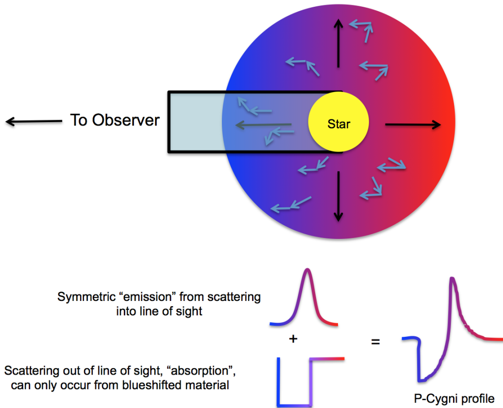
FIGURE 2.1: Diagram showing how an expanding envelope or wind presenting significant line opacity around a continuum source leads to the formation of P-Cygni profiles. The black arrows denote the outflow direction and the blue arrows typical scattering interactions.
