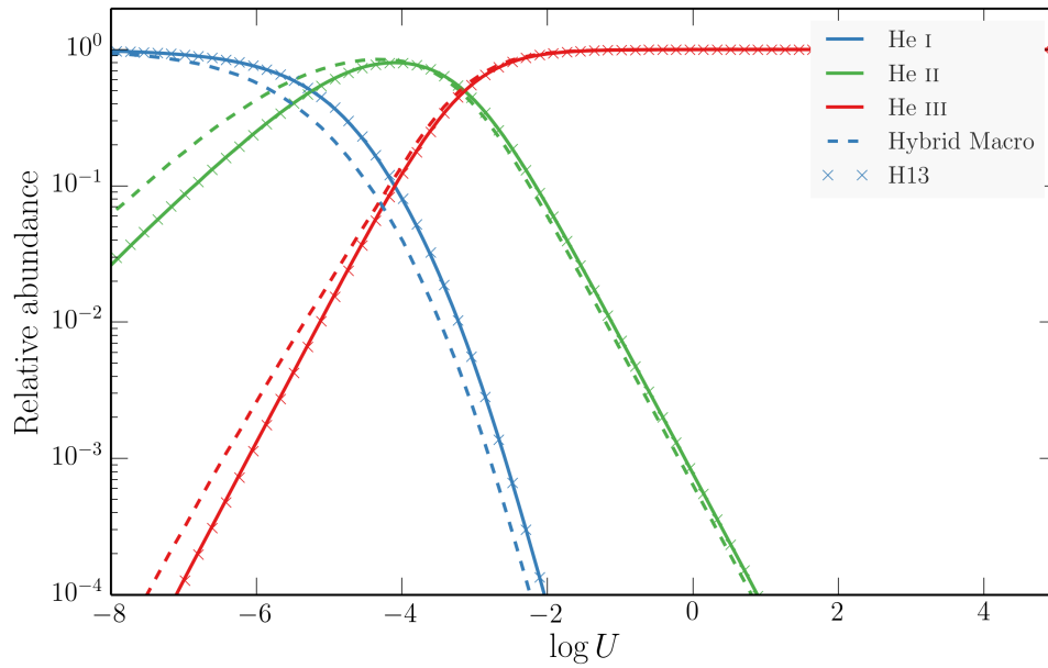
FIGURE 3.10: As figure 3.9, but for Helium.
