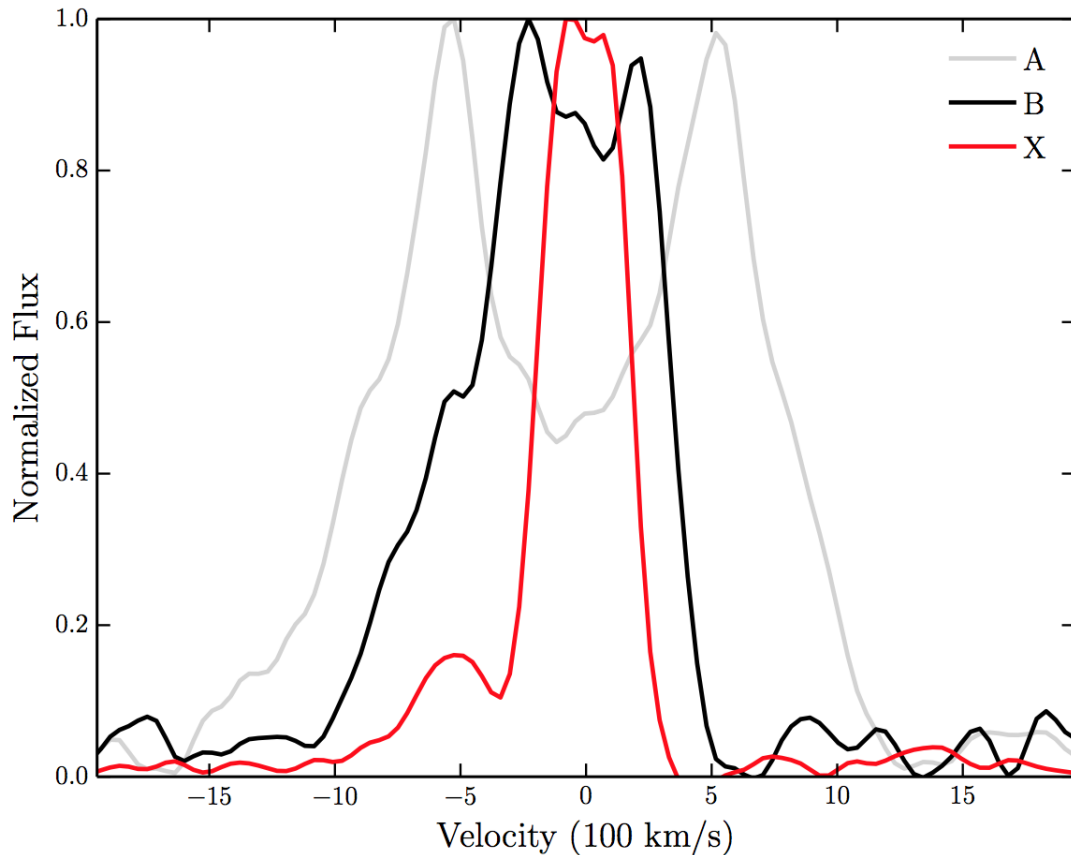
FIGURE 4.10: H\alpha line profiles, normalized to 1, plotted in velocity space for three models with varying kinematic properties, computed at an inclination of 80^\circ . The benchmark model and the improved optical model described in section 4.3 are labeled as A and B respectively, and a third model (X) which has an increased acceleration length of R_v = 283.8 R_{WD} , and \alpha = 4 is also shown. The x -axis limits correspond to the Keplerian velocity at 4 R_{WD} , the inner edge of the wind. There is a narrowing of the lines, and a single-peaked line in model X. This is not due to radial velocity shear (see section 4.3.3).
