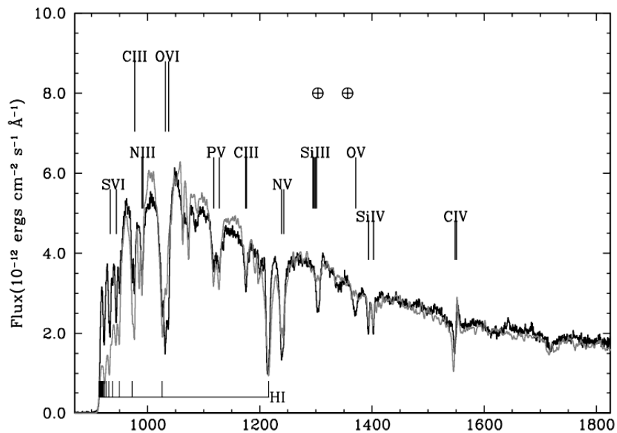
FIGURE 2.3: Credit: Long & Knigge 2002. UV spectrum of Z Cam (black), compared to a synthetic spectrum from MCRT simulations (grey).
