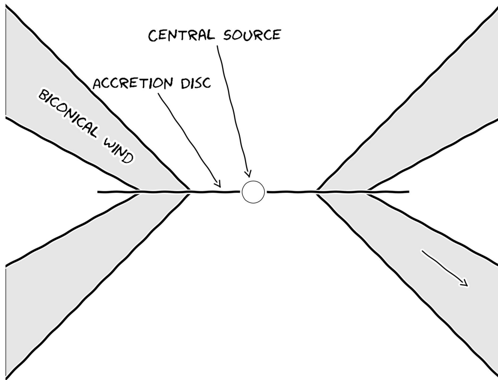
FIGURE 1.15: Occam's quasar. How far can this general picture take us when trying to explain the behaviour of quasars and other accreting compact objects?
