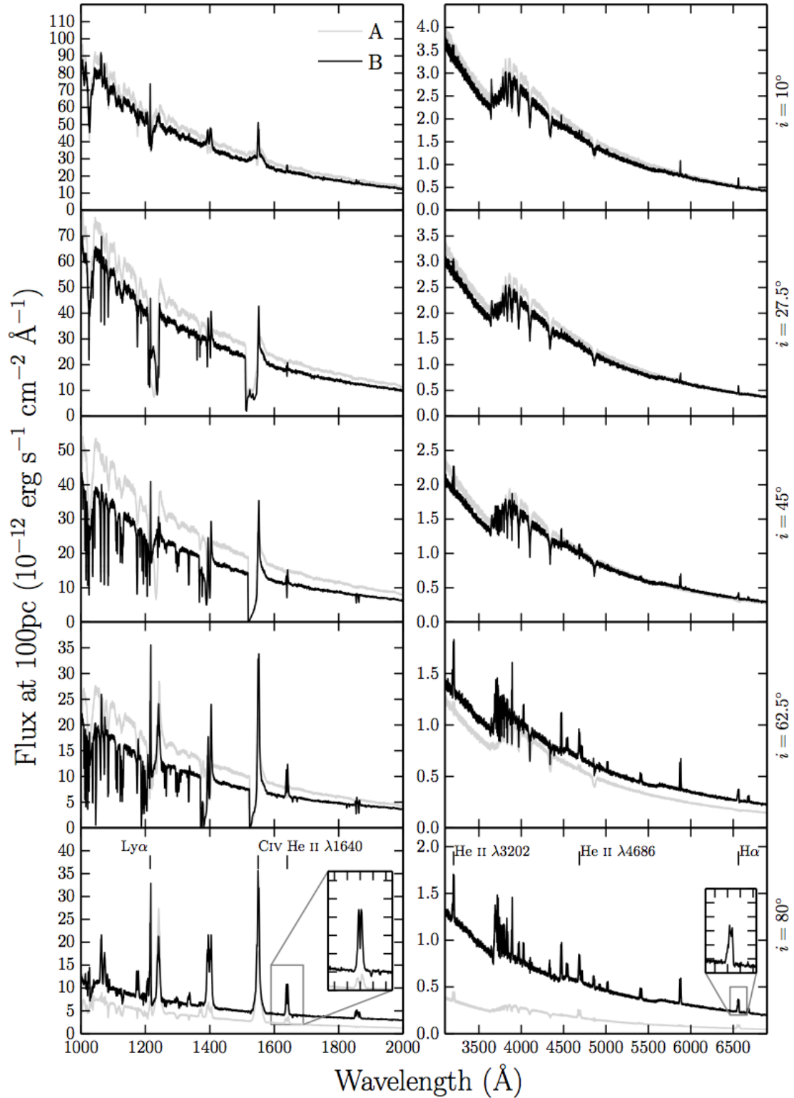
FIGURE 4.7: UV (left) and optical (right) synthetic spectra for model B computed at sightlines of 10, 27.5, 45, 62.5 and 80 degrees. Model A is shown in grey for comparison. The inset plots show zoomed-in line profiles for He II 1640 Å and H \alpha . The Balmer and He are double-peaked, albeit with narrower profiles. Strong He II 4686 Å emission can be seen, as well as a trend of a deeper Balmer jump with decreasing inclination.
