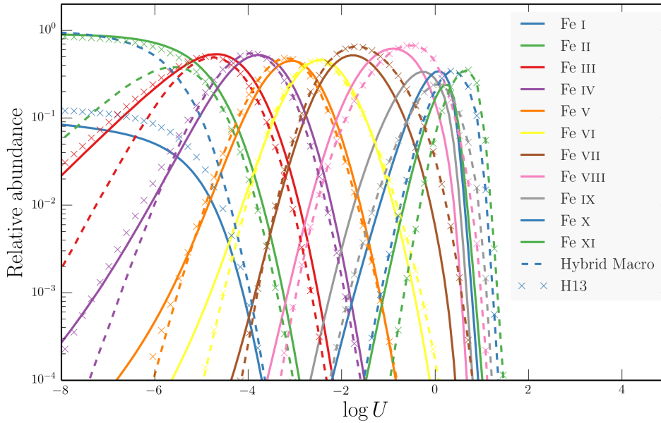
FIGURE 3.14: As figure 3.9, but for the first 11 ionization stages of Iron.
