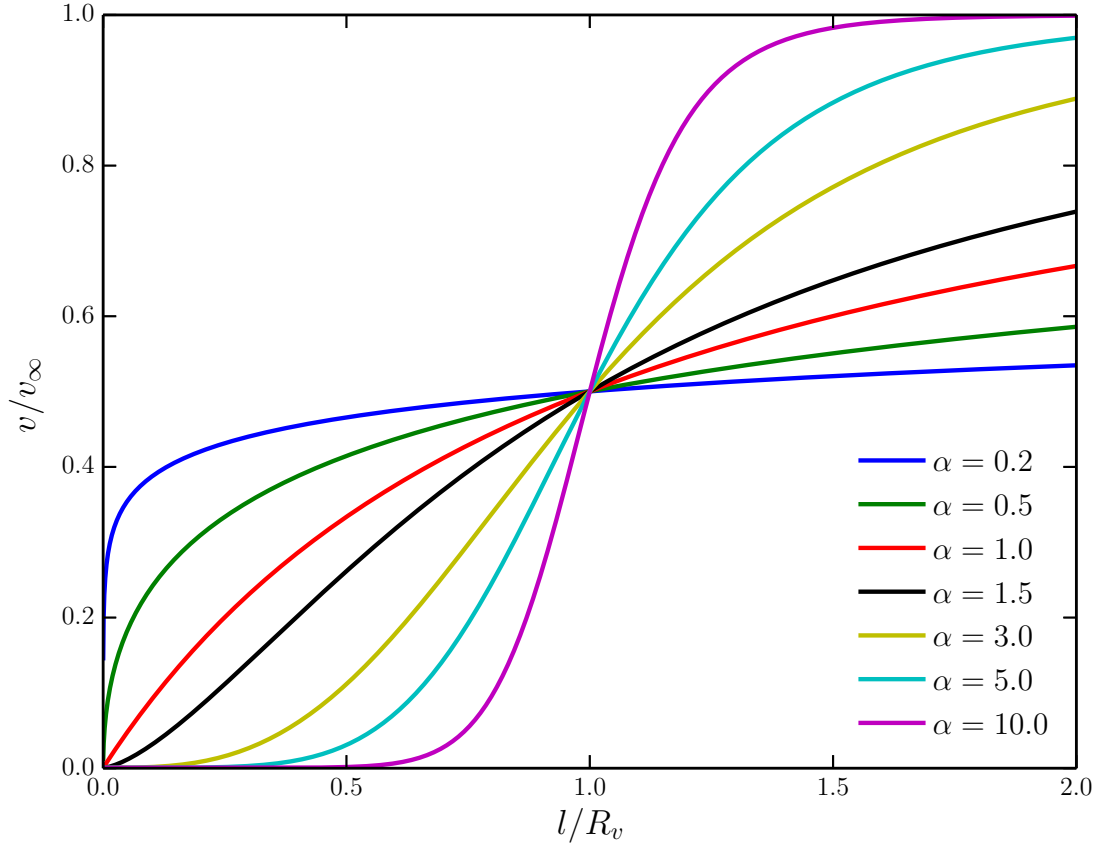
FIGURE 2.15: The SV93 velocity law for various values of the acceleration exponent, \alpha .
