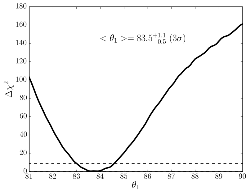
FIGURE 6.6: \Delta\chi^2 as a function of maximum angle, \theta_1 , calculated in steps of 0.1^\circ . The choice for \mu_* and \sigma_* is left free in each case. The dotted line marks the 3\sigma confidence interval.
