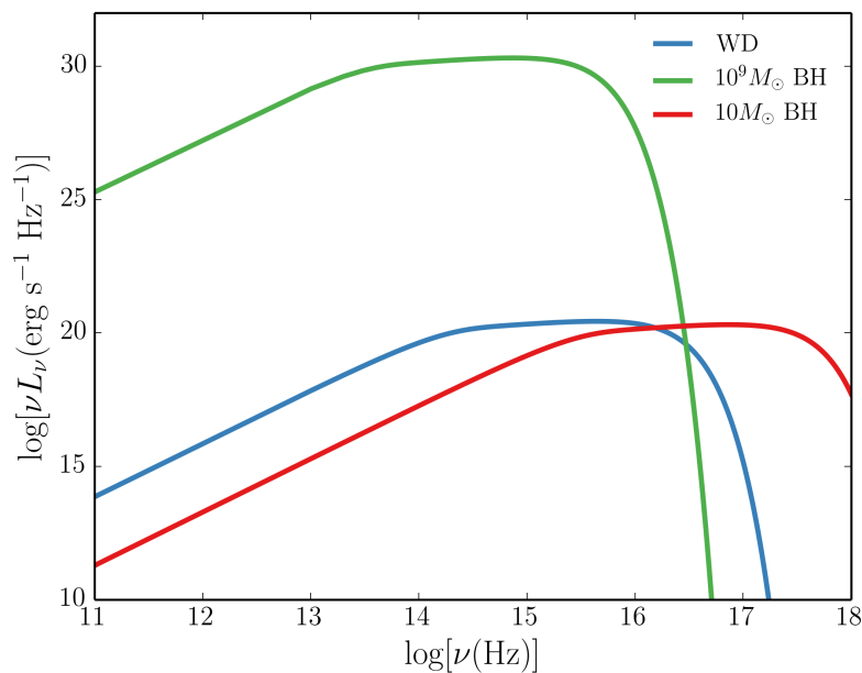
FIGURE 1.4: Accretion disc SEDs for three different compact objects, corresponding roughly to a quasar, an XRB and a CV. The SEDs are computed via an area-weighted sum of blackbodies with effective temperatures governed by equation 1.18, and the \nu^{1/3} shape in the middle of the spectra can be seen.
