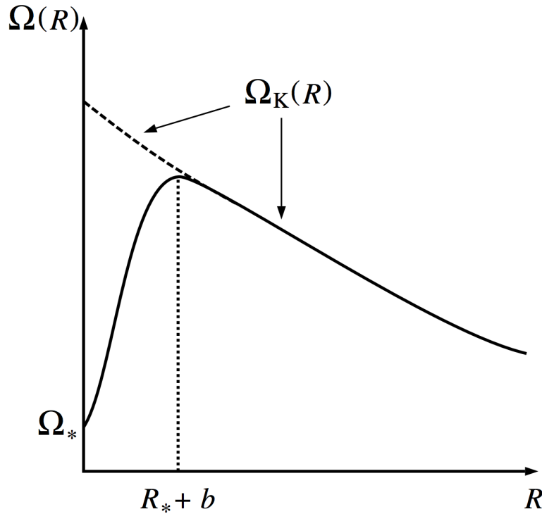
FIGURE 1.2: Credit: Frank et al. 2002. Angular velocity as a function of radius in an accretion disc around a rotating compact object with angular velocity \Omega_* . \Omega_K is the Keplerian angular velocity. This graph also helps explain why there is a turnover in the temperature-radius relation, as D(R) is proportional to the square of the derivative of this quantity. The boundary condition responsible for this turnover is briefly discussed in the text.
