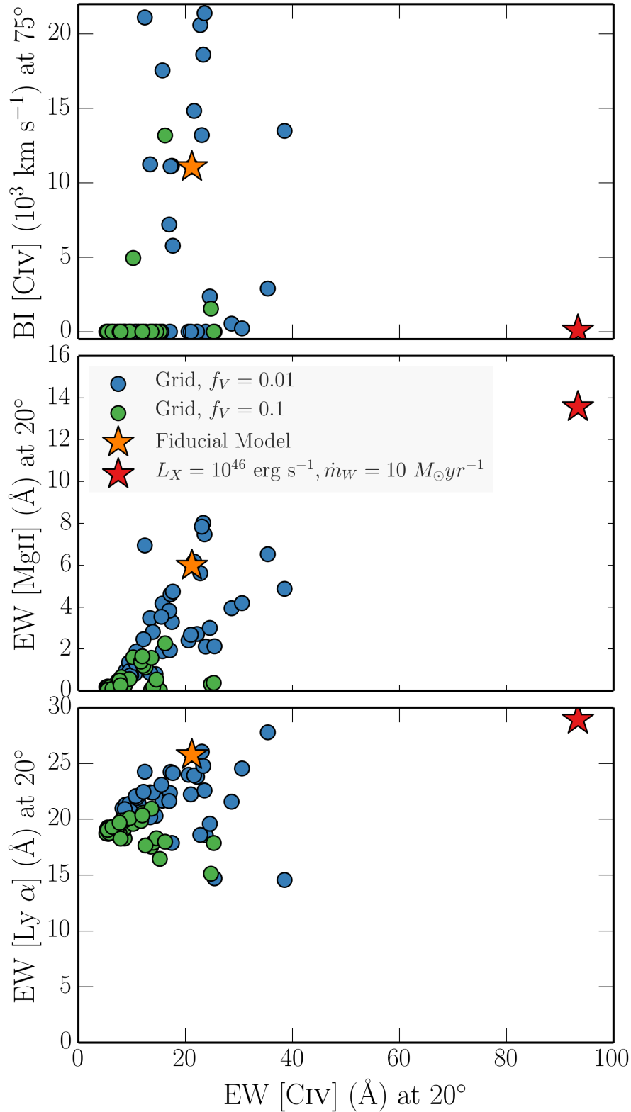
FIGURE 5.11: The EW of the C IV 1550 \text{\AA} line at 20^\circ plotted against a) the BI of C IV 1550 \text{\AA} at 75^\circ , b) the EW of the Mg II 2800 \text{\AA} line at 20^\circ and c) the EW of Ly \alpha at 20^\circ . The circles correspond to the simulation grid for two different values of f_V , and the fiducial model is marked with an orange star. I also show a higher X-ray luminosity model and a higher mass loss rate with a red star.
