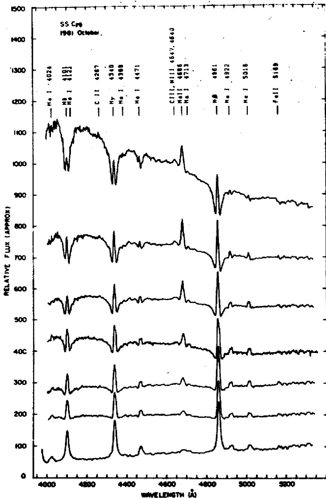
FIGURE 1.9: Credit: Hessman et al. 1984 / Dhillon et al. 1996. Spectra of SS Cyg during an outburst cycle, showing the evolution from minimum to maximum light. The rise is characterised by the appearance of an optically thick accretion disc spectrum. The flux scale is approximate.
