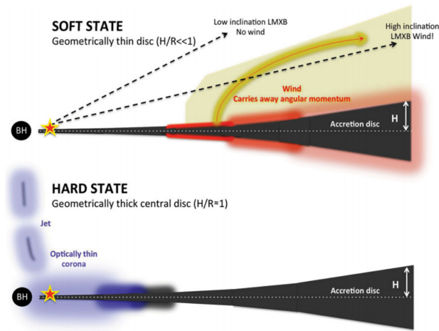
FIGURE 2.5: Credit: Ponti et al. 2012. A cartoon illustrating the expected geometry of the disc and outflows in LMXBs in the soft and hard states.
