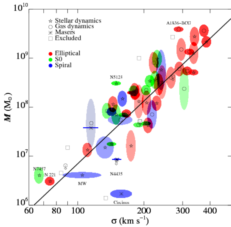
FIGURE 2.16: Credit: Gultekin et al. 2009. The M_{BH} - \sigma_* correlation.
