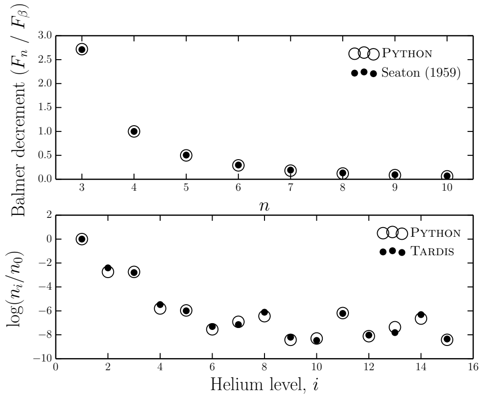
FIGURE 3.15: Top Panel: ‘Case B’ Balmer decrements computed with PYTHON compared to analytic calculations by Seaton (1959). Both calculations are calculated at T_e = 10,000\text{K} . Bottom Panel: a comparison of He I level populations (the most complex ion we currently treat as a macro-atom) between PYTHON and TARDIS models. The calculation is conducted in thin shell mode with physical parameters of n_e = 5.96 \times 10^4 \text{ cm}^{-3} , T_e = 30,600\text{K} , T_R = 43,482\text{K} and W = 9.65 \times 10^{-5} .
