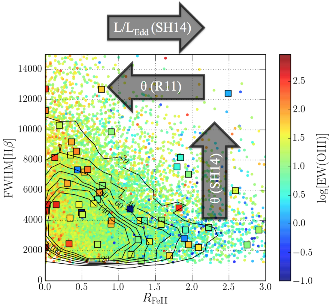
FIGURE 6.10: Eigenvector 1 for LoBAL and non-BAL quasars. FWHM of the H\beta line plotted against the relative iron strength, R_{\text{FeII}} . The colour coding corresponds to the EW of [O\text{ III}] 5007 \text{ \AA} . The dots mark all quasars from sample A, while the squares mark those with Mg II LoBALs. A few of the Mg II LoBALQSOs are missing due to their lack of \text{FWHM}[H\beta] measurements. The arrows show the approximate direction of the expected inclination ( \theta ) trend under both the SH14 and R11 interpretations, and the expected trend in Eddington fraction ( L/L_{\text{Edd}} ) from SH14 only.
