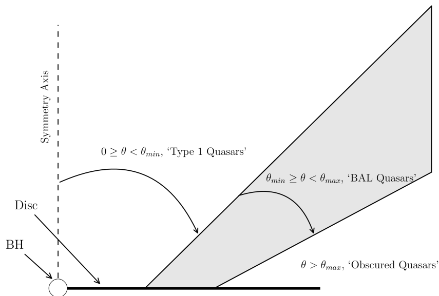
FIGURE 6.7: The geometry of the toy model used to carry out the Monte Carlo simulations.
