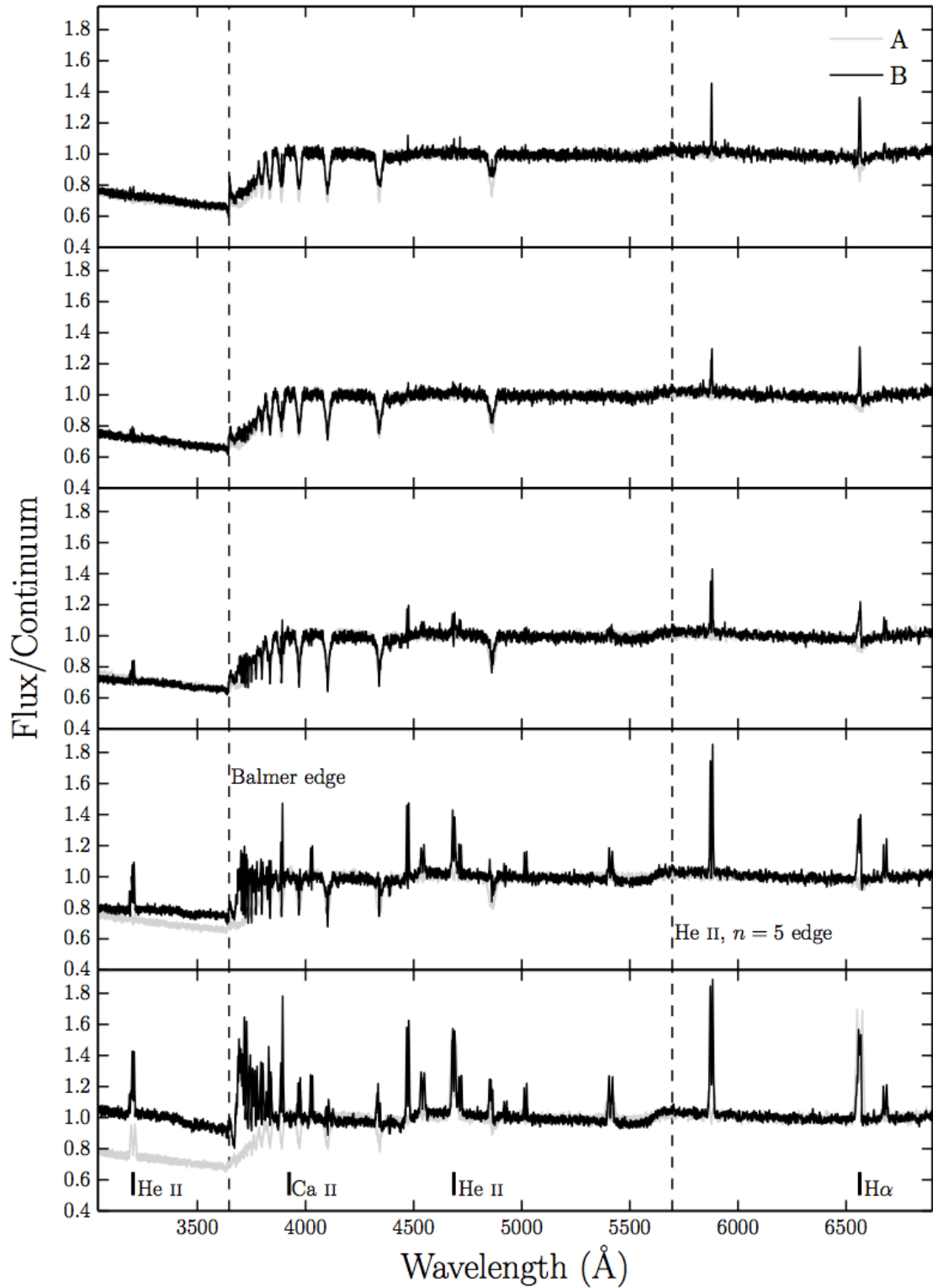
FIGURE 4.8: Synthetic optical spectra from model B computed for sightlines of 10, 27.5, 45, 62.5 and 80 degrees. Model A is shown in grey for comparison. In these plots the flux is divided by a polynomial fit to the underlying continuum redward of the Balmer edge, so that line-to-continuum ratios and the true depth of the Balmer jump can be shown.
