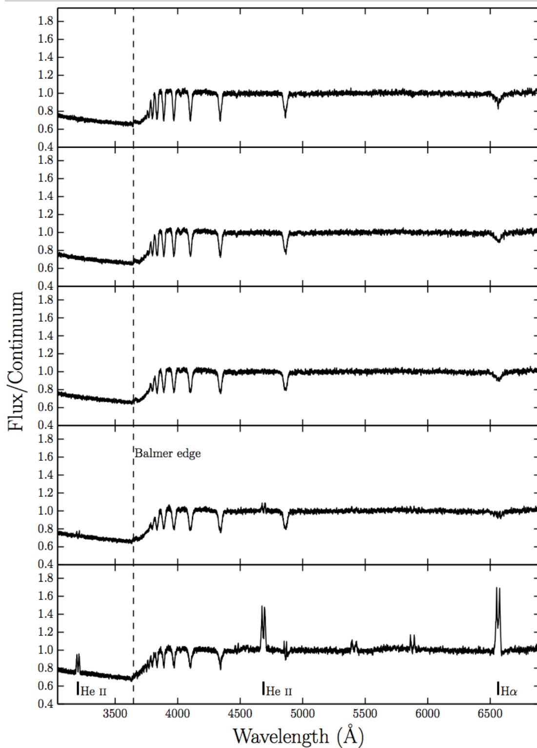
FIGURE 4.5: Synthetic optical spectra from model A computed for sightlines of 10, 27.5, 45, 62.5 and 80 degrees. In these plots the flux is divided by a polynomial fit to the underlying continuum redward of the Balmer edge, so that line-to-continuum ratios and the true depth of the Balmer jump can be shown.
