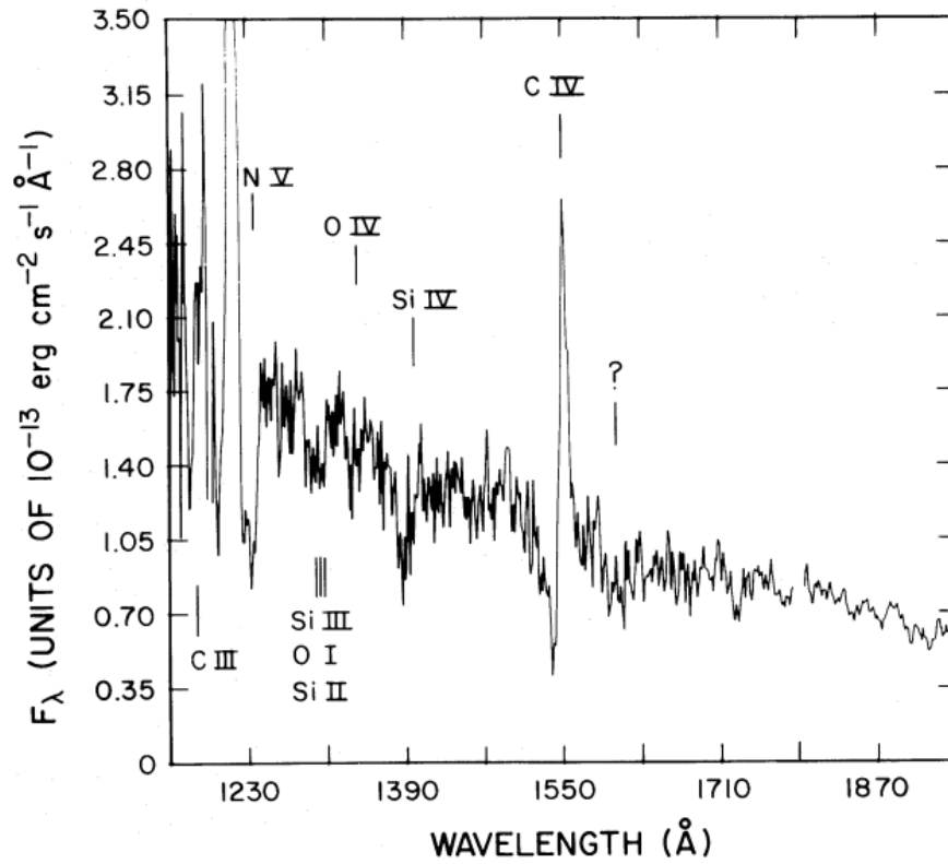
FIGURE 2.2: Credit: Cordova & Mason 1982. UV spectrum of the DN TW Vir during outburst. The P-Cygni profiles can be seen clearly, demonstrating that a strong, fast outflow is present in the system.
