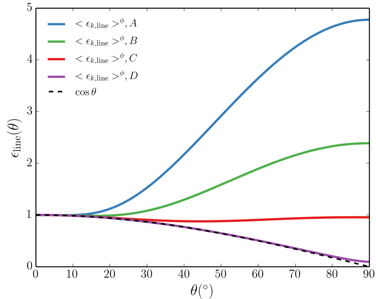
FIGURE 6.15: The azimuthally-averaged line angular emissivity function, \bar{\epsilon}_{k,\text{line}} , from a Keplerian disc as a function of inclination angle for the four models shown in table 6.1. The model parameters are the values of H/R , v_k and v_{th} . The zero Keplerian velocity shear case, \epsilon_{0,\text{line}}(\theta) = \cos \theta (dotted line), is also shown. Unless the disc is very thin ( H/R \sim 0.001 ), \bar{\epsilon}_{k,\text{line}} shows large deviations from \cos \theta .
