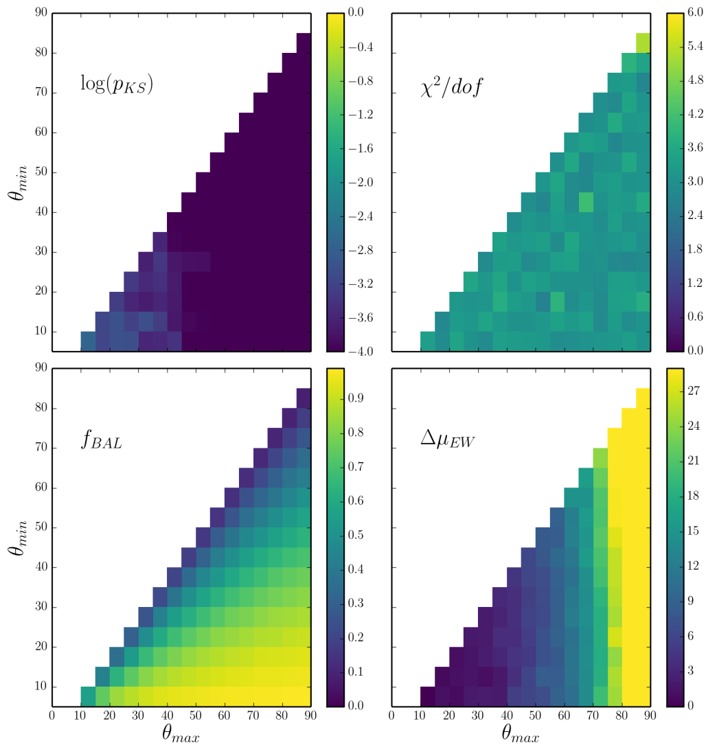
FIGURE 6.9: Heat map showing the results of the MC simulation described in section 6.4.2, but this time conducted with a Log-normal intrinsic distribution. The quantities shown are the same as in Fig. 6.8. Note the different scale for the colour coding of the \chi^2/dof panel (upper right).
