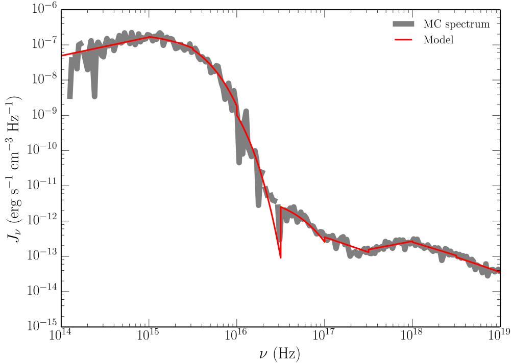
FIGURE 3.5: An example of a modeled spectrum in PYTHON compared to the recorded MC spectrum, from an individual cell in an AGN model.
