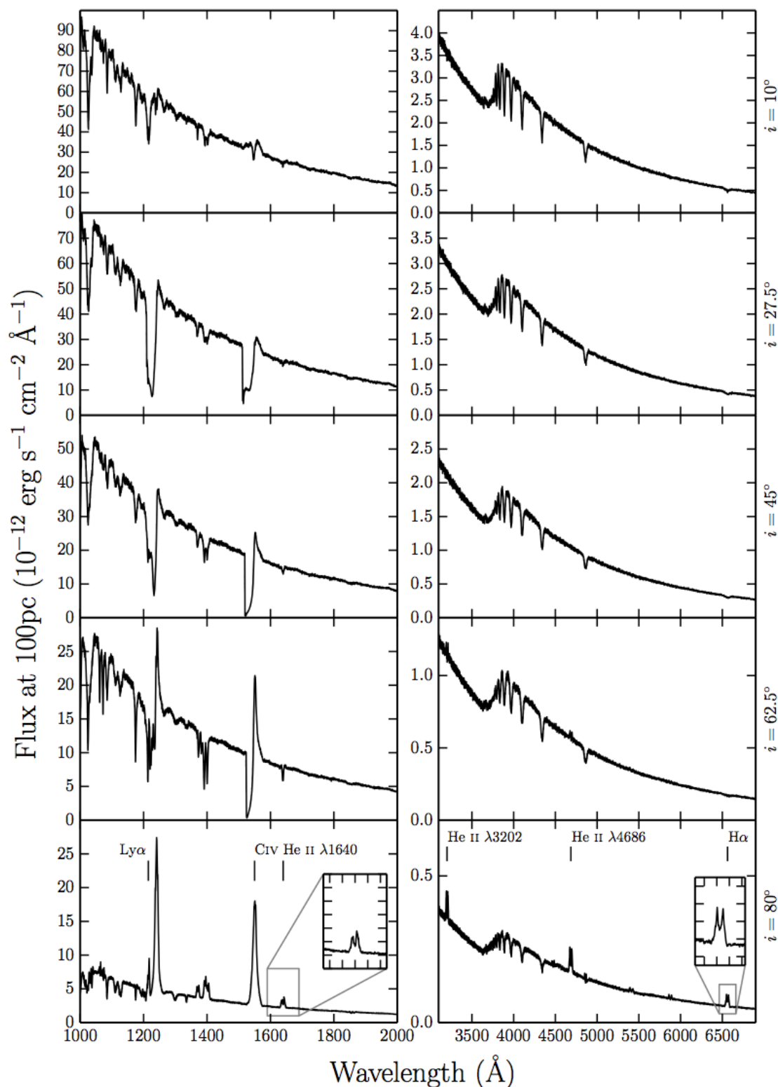
FIGURE 4.4: UV (left) and optical (right) synthetic spectra for model A, the benchmark model, computed at sightlines of 10, 27.5, 45, 62.5 and 80 degrees. The inset plots show zoomed-in line profiles for He II 1640 Å and H \alpha . Double-peaked line emission can be seen in He II 1640 Å, He II 4686 Å, H \alpha and some He I lines, but the line emission is not always sufficient to overcome the absorption cores from the stellar atmosphere models.
