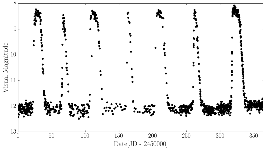
FIGURE 1.8: Data: AAVSO. A year in the life of SS Cyg, showing the characteristic repeated outbursts and periods of quiescence typical of a DN. SS Cyg has been undergoing this activity since it was first observed in 1896.
