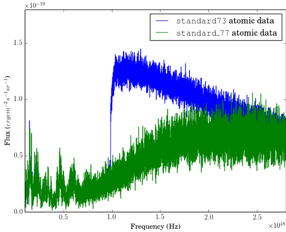
FIGURE 3.8: A comparison of the soft X-ray regime of the H13 model, with two different datasets. standard73 is the dataset with old, unextrapolated cross-sections and standard77 instead includes extrapolated cross-sections as described in the text.
