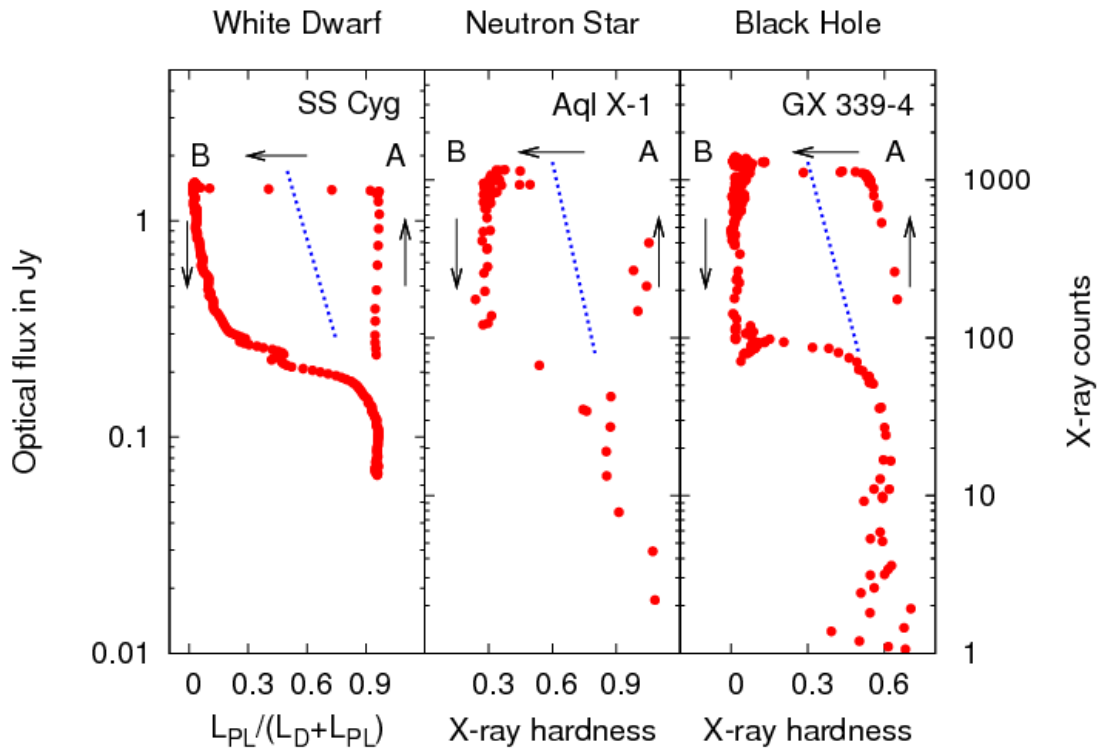
FIGURE 1.16: Credit: Kording et al. 2008. Hardness-intensity diagrams for three types of accreting compact objects: the dwarf nova SS Cyg (left), in addition to neutron star (middle) and black hole (right) LMXBs. The dotted line shows the ‘jet line’ in LMXBs and the arrows show the expected temporal evolution of the system. For SS Cyg the x -axis shows the fraction of the hard X-ray power law component in the system compared to the luminosity of the combined luminosity of disc and power law. This quantity is analogous to the X-ray hardness in LMXBs.
