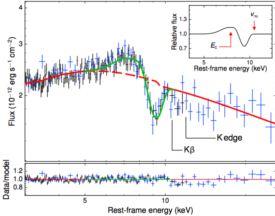
FIGURE 2.8: Credit: Nardini et al. 2015. X-ray spectrum of PDS 456 fitted with a P-Cygni profile from a spherical outflow model. XMM-Newton data is shown in black with two combined NuStar observations in blue.
