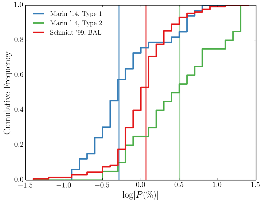
FIGURE 6.13: Cumulative distribution functions of the histograms shown in Fig. 6.12 for BAL quasars from Schmidt et al. (1999) together with the Marin et al. (2014) AGN sample. The colour-coding and x -axis scale are the same as Fig. 6.12. The translucent vertical lines mark the median value in each sample.
