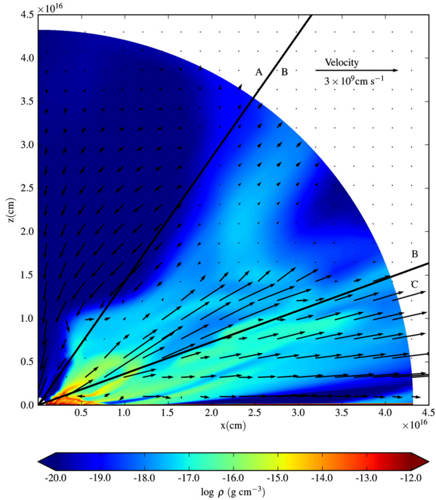
FIGURE 2.13: Credit: Higginbottom et al. 2014. A snapshot of the PK04 model. Colours shows the density and arrows show the velocity of the flow. The radial lines separate three areas described by H14.
