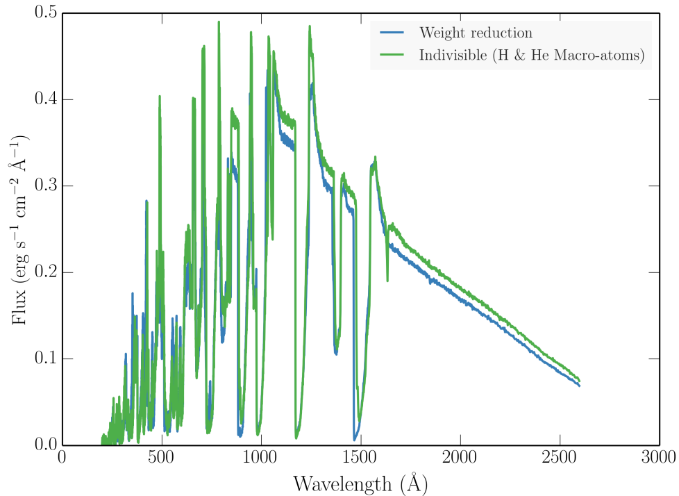
FIGURE 3.17: A comparison between weight reduction and line transfer mode. The model is the H13 fiducial BALQSO model – agreement is generally even better for CV models.
