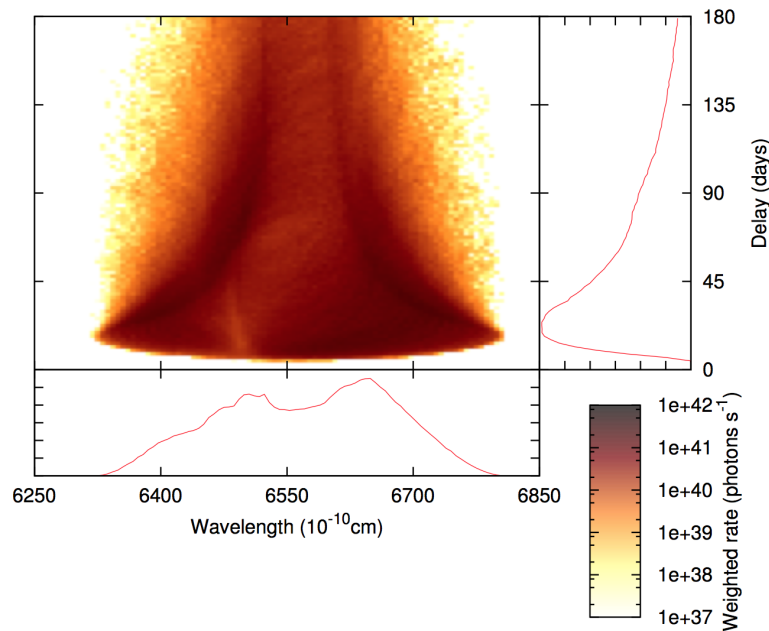
FIGURE 7.2: Credit: Sam Mangham. Velocity-resolved transfer function for H \alpha from the fiducial quasar model presented in chapter 5. The transfer function is for a viewing angle of 40^\circ .
