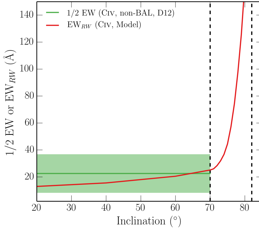
FIGURE 5.12: EW_{RW} as a function of inclination in the fiducial model, compared to 1/2 EW from the quasar sample of Di Pompeo et al. (2012; D12). The shaded region corresponds to the standard deviation of the D12 sample.
