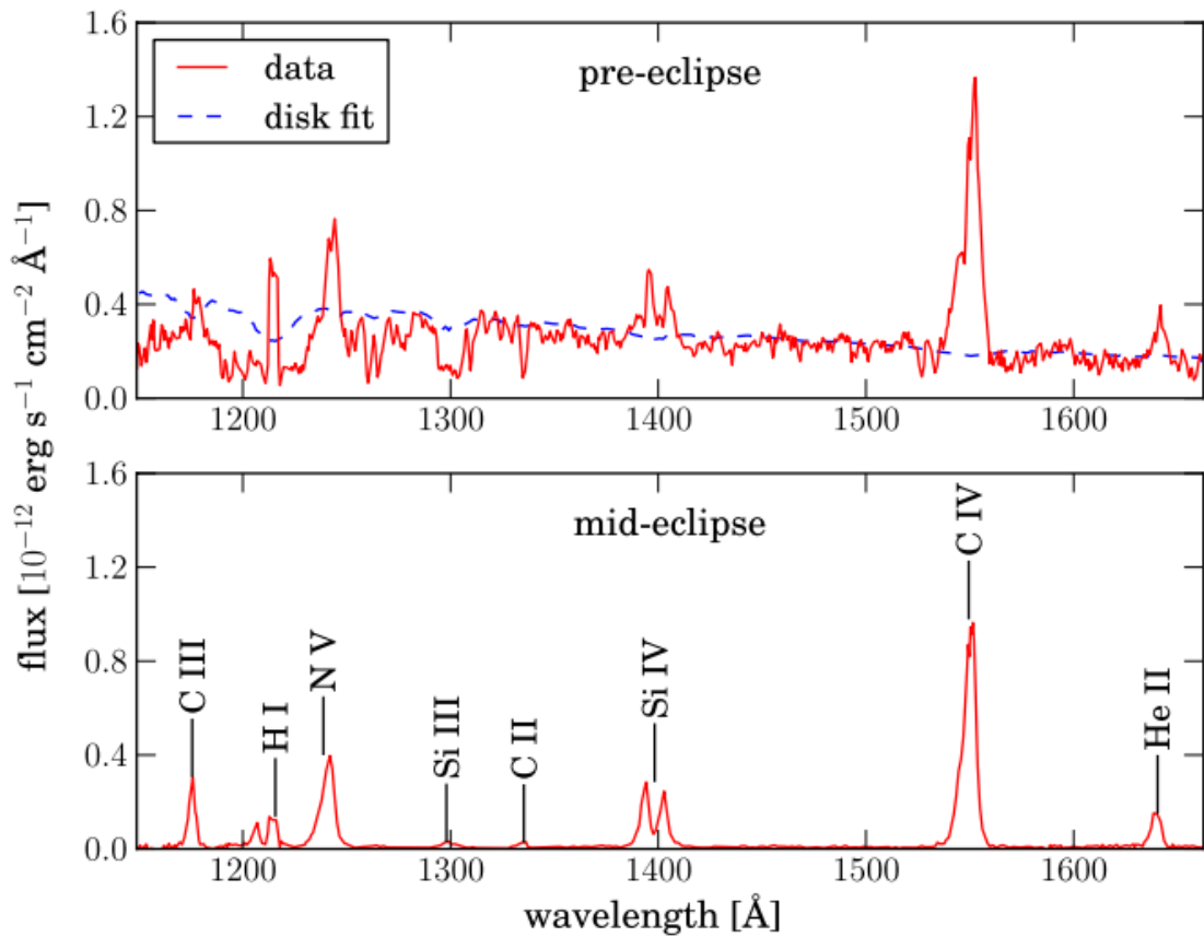
FIGURE 1.10: Credit: Noebauer et al. 2010. UV spectrum of RW Tri in and out of eclipse, showing strong lines in C IV 1550 Å and Ly \alpha , among others.
