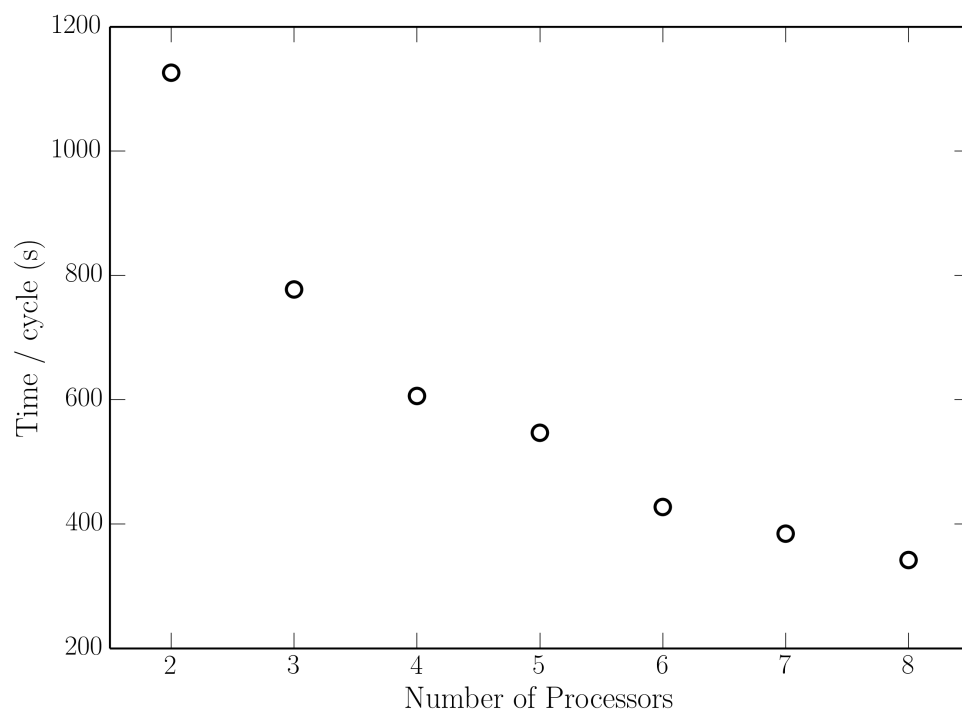
FIGURE 3.19: Total runtime per cycle for an AGN run as a function of the number of processors.
